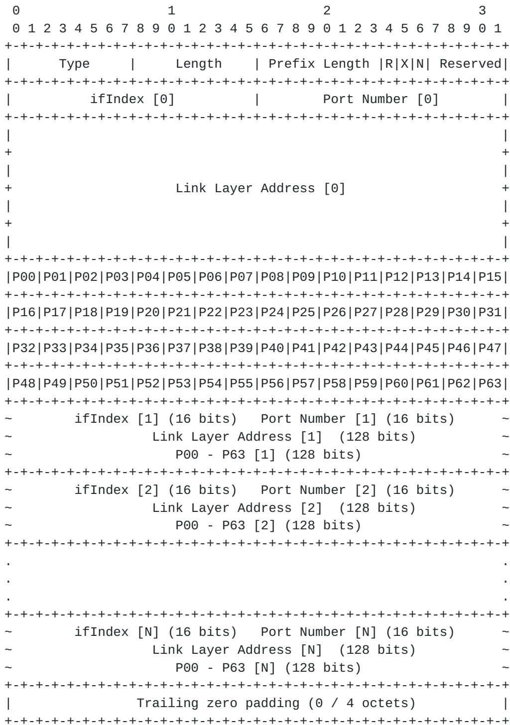
Figure 4: AERO Source/Target Link-Layer Address Option (S/TLLA0) Format
