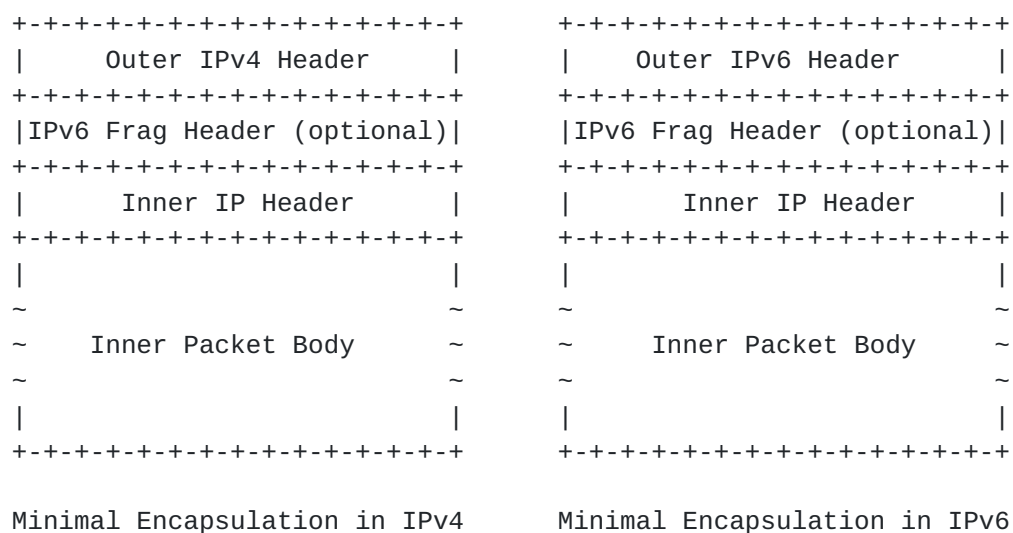
Figure 7: Minimal Encapsulation Format using IP-in-IP
