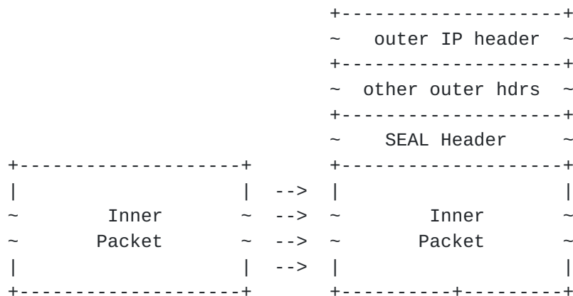
Figure 1: SEAL Encapsulation
