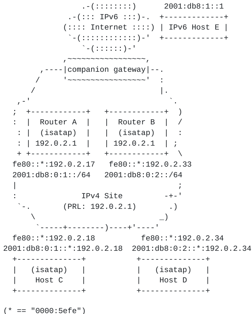
Figure 2: Example ISATAP Network Topology using Individual Prefix Model
