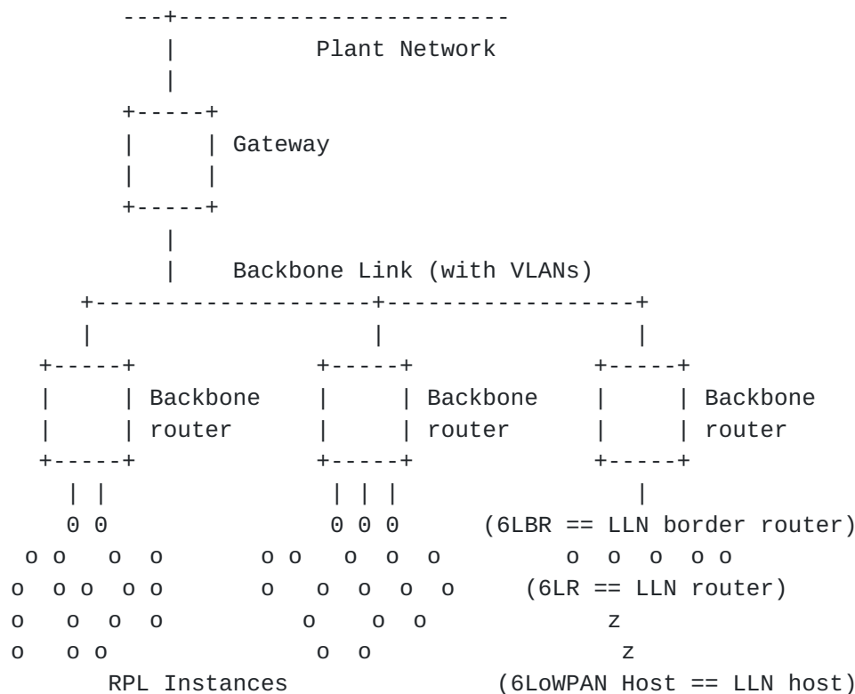
Figure 1: 6TiSCH architecture
