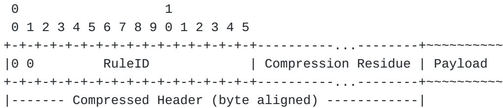
Figure 3: SCHC Compressed Packet
