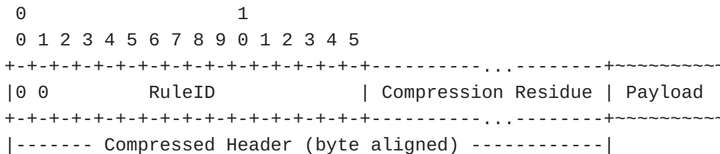
Figure 3: SCHC Compressed Packet
