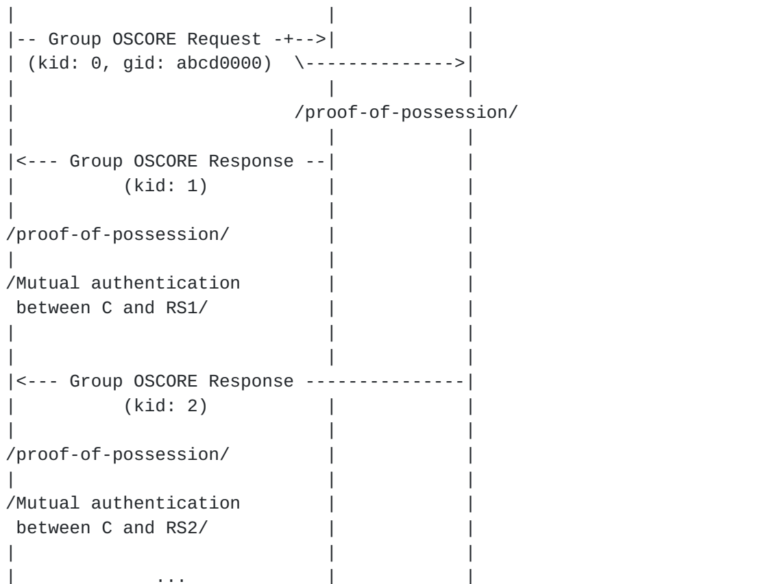
Figure 1: Protocol Overview.
