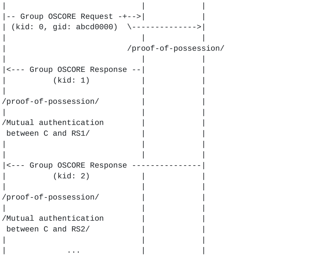
Figure 1: Protocol Overview.
