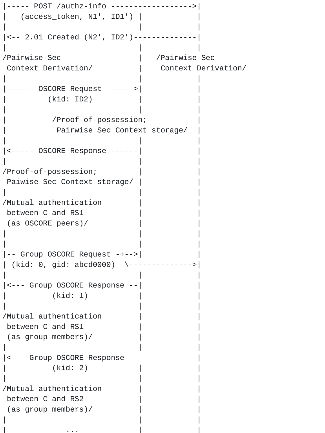
Figure 8: Protocol Overview.
