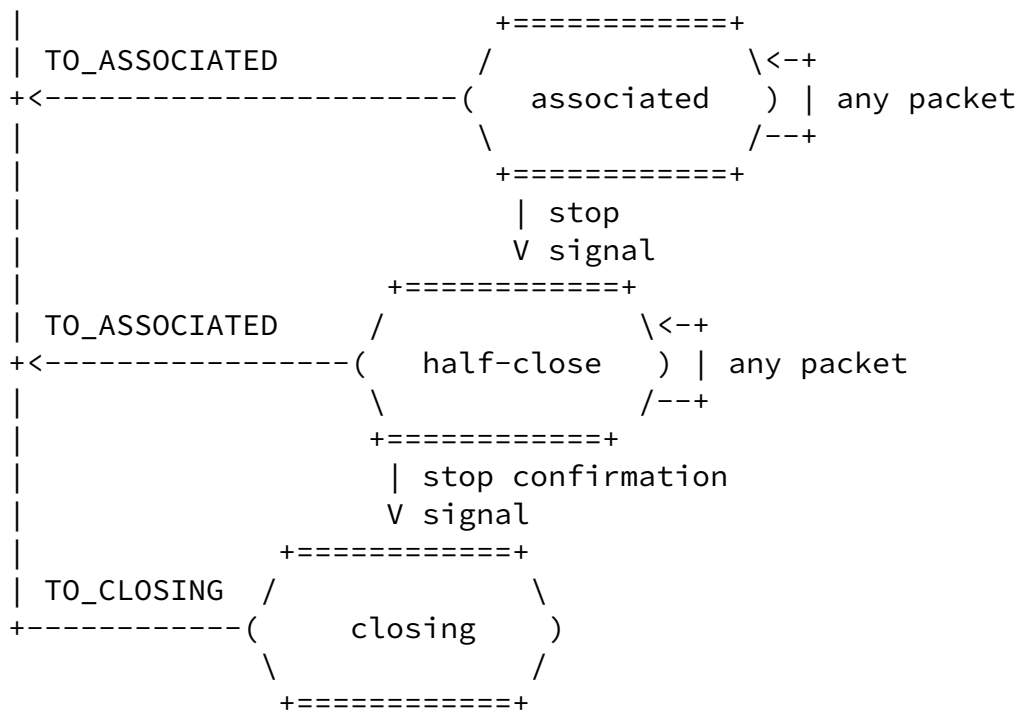
Figure 1: Transport-Independent State Machine for Stateful On-Path Devices
