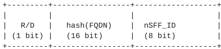
Figure 12: Registration packet format
