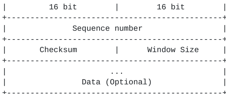
Figure 10: Transport protocol data packet format
