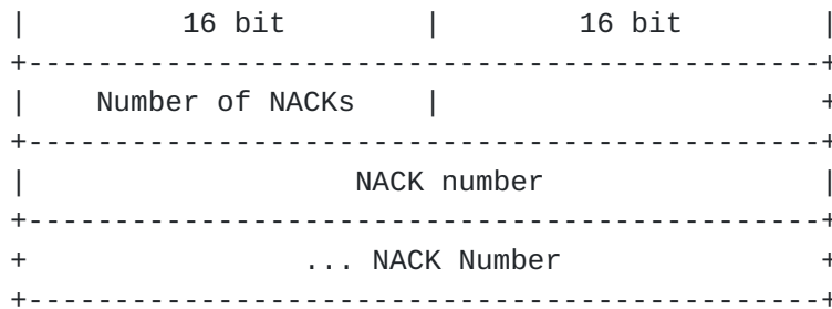
Figure 11: Transport protocol NACK packet format
