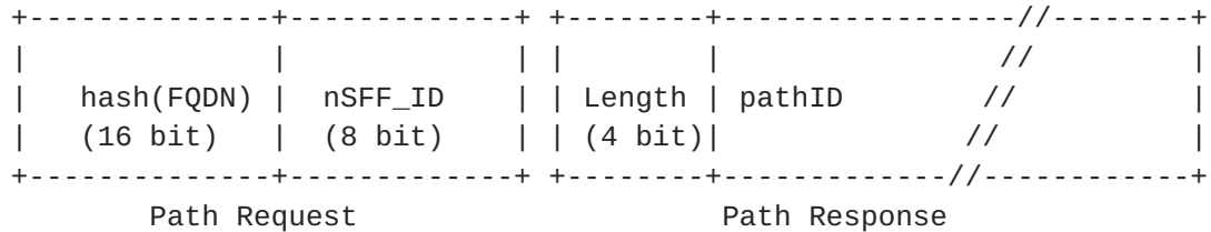
Figure 13: Discovery packet format
