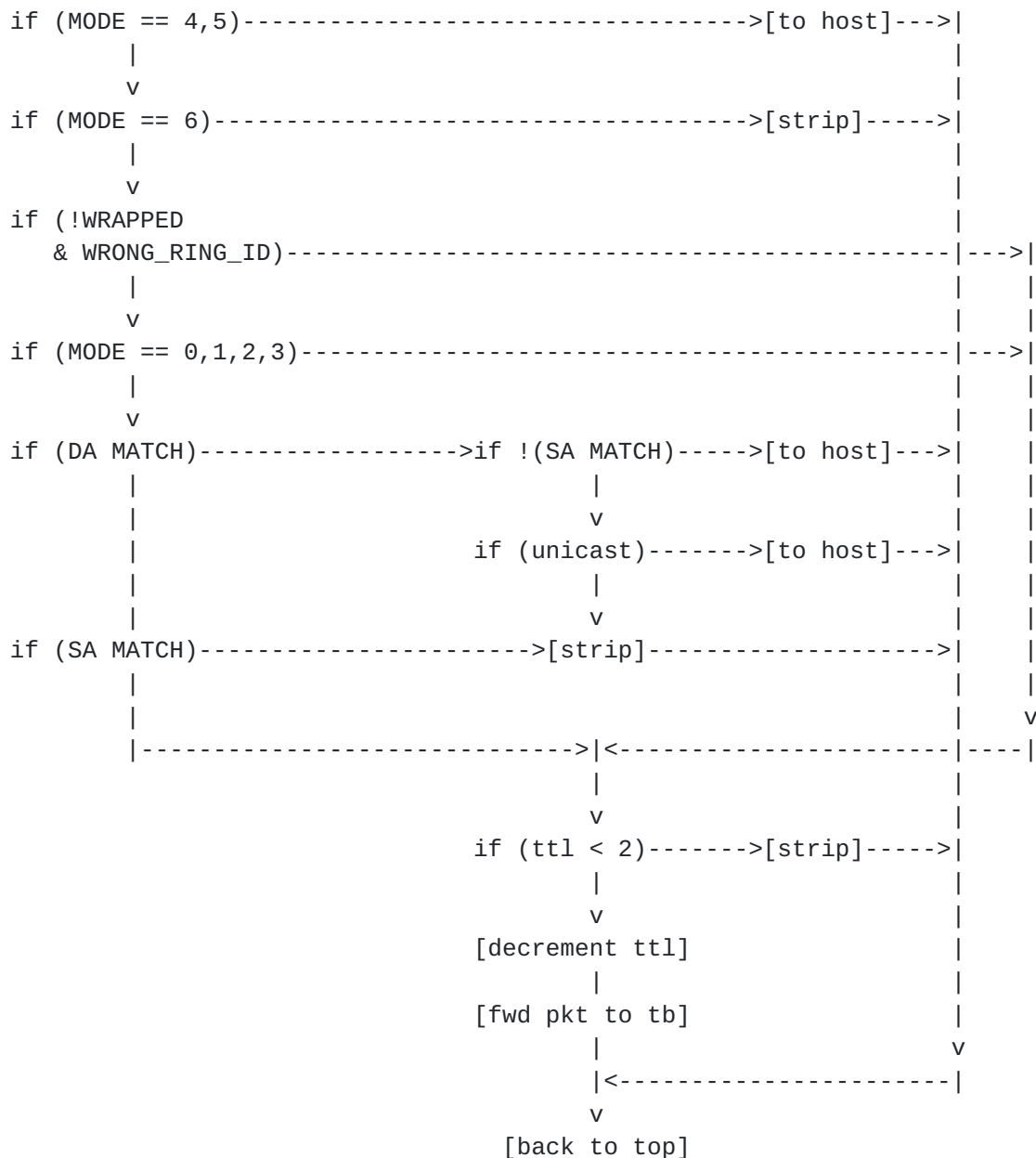
FIGURE 16. SRP Receive Flowchart (Packet node)
