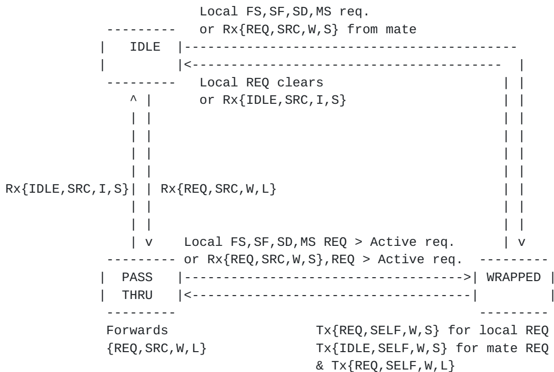
FIGURE 20. Simplified State Transitions Diagram
