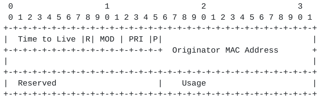
FIGURE 10. Usage Packet Format
