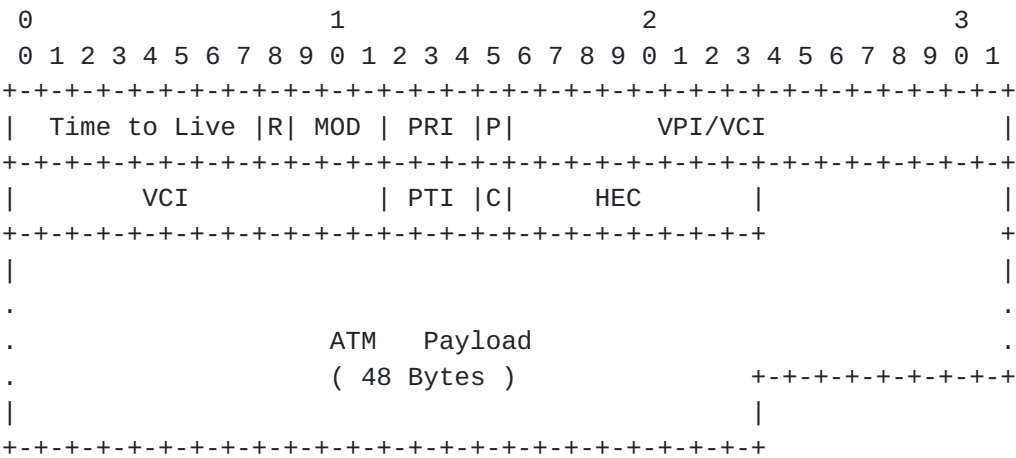
FIGURE 9. SRP Cell Format
