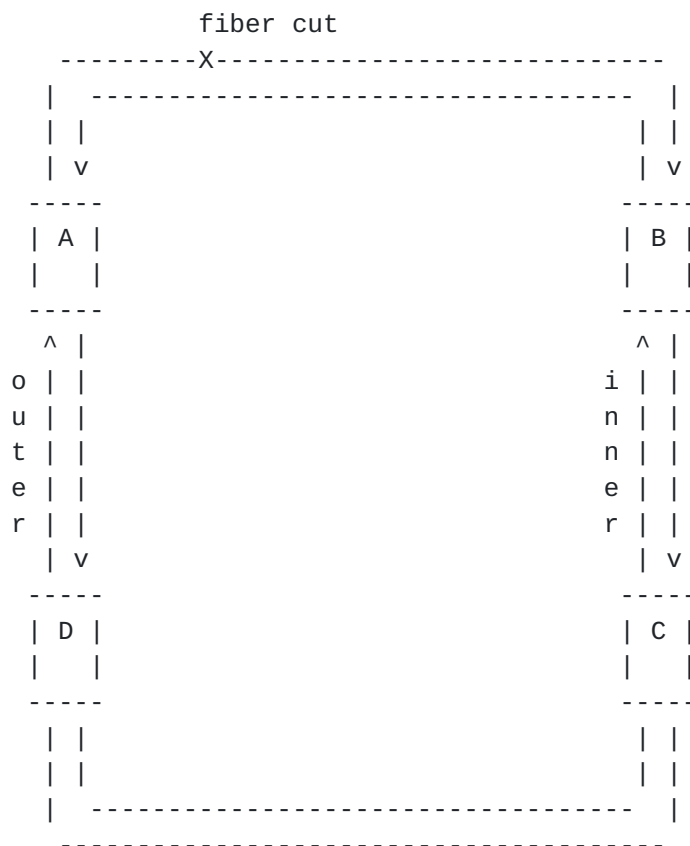
FIGURE 21. An SRP Ring with outer ring fiber cut
