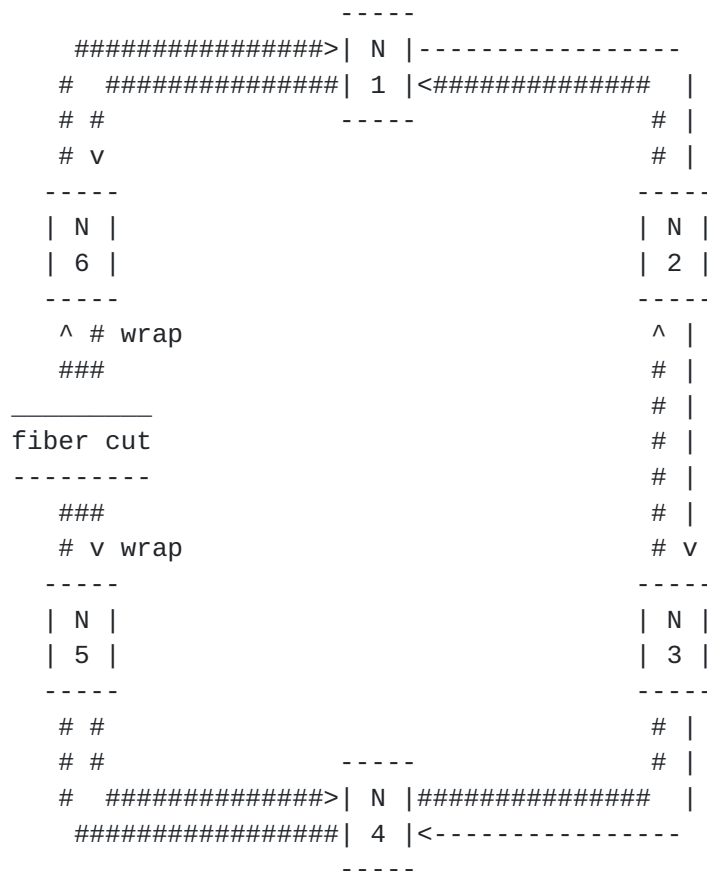
FIGURE 5. Data path after the wrap, N4 -&gt; N1
