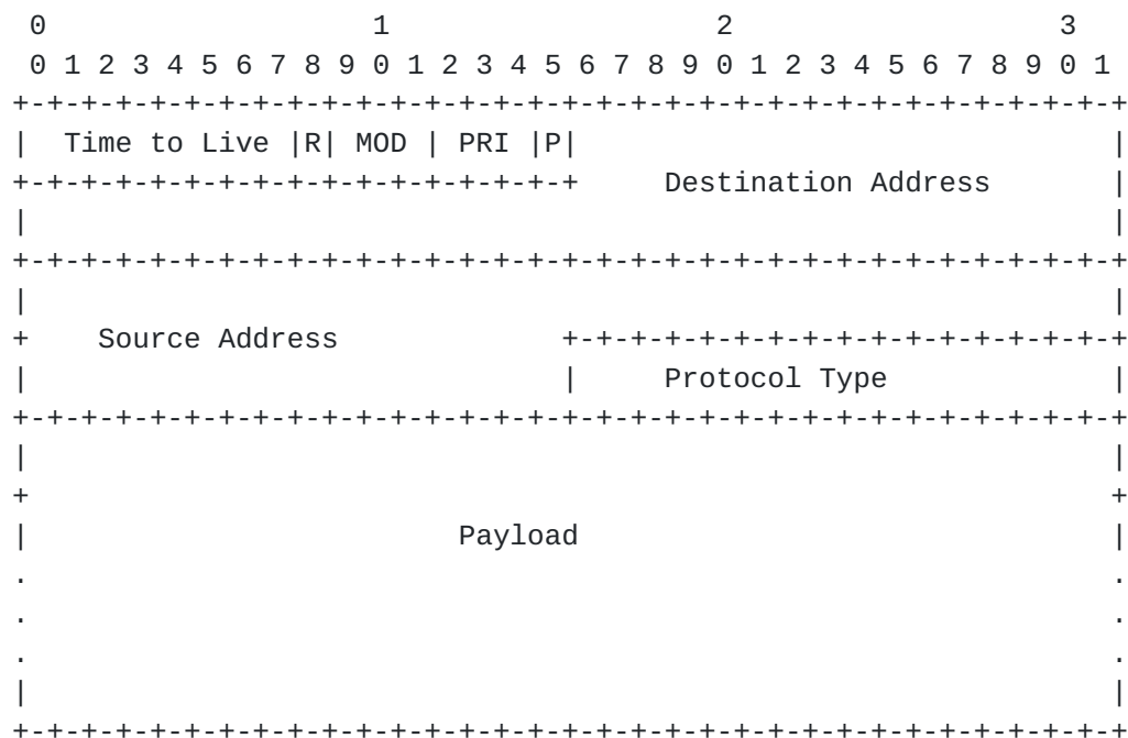
FIGURE 8. Detailed Packet Header Format
