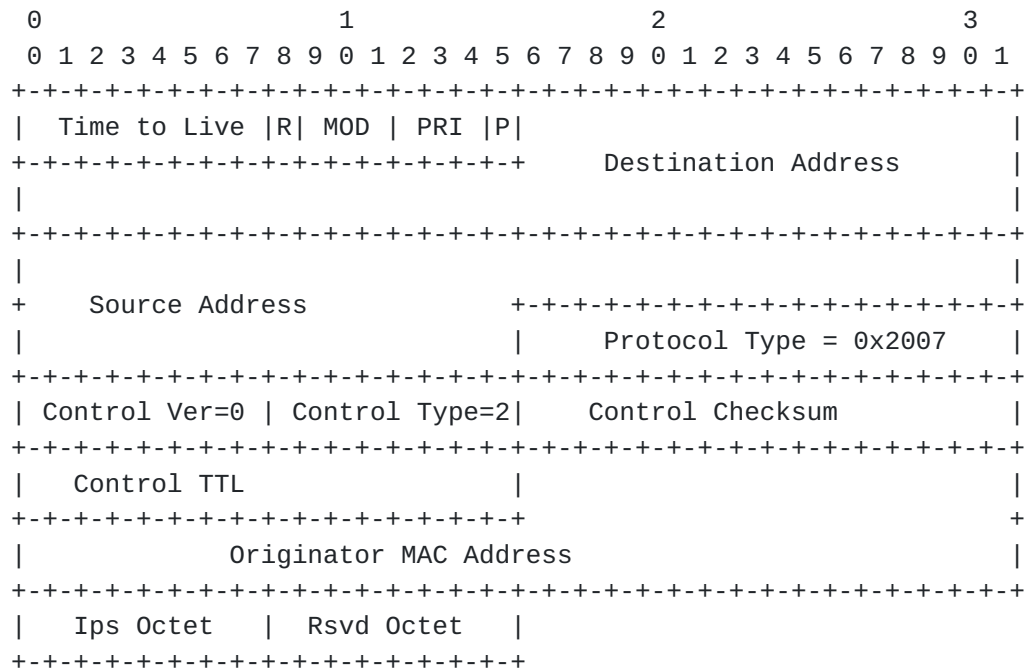
FIGURE 14. IPS Packet Format
