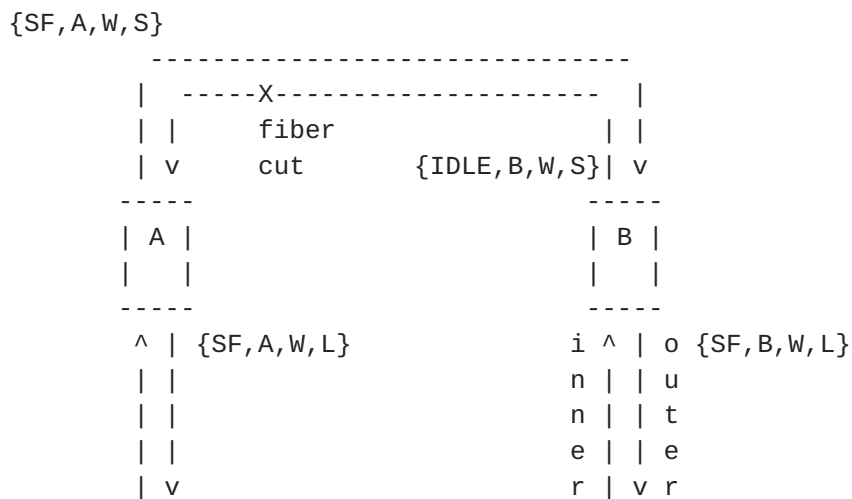
FIGURE 19. SRP IPS Signaling
