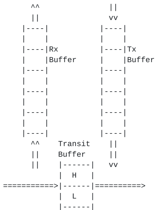
FIGURE 3. Transit buffer
