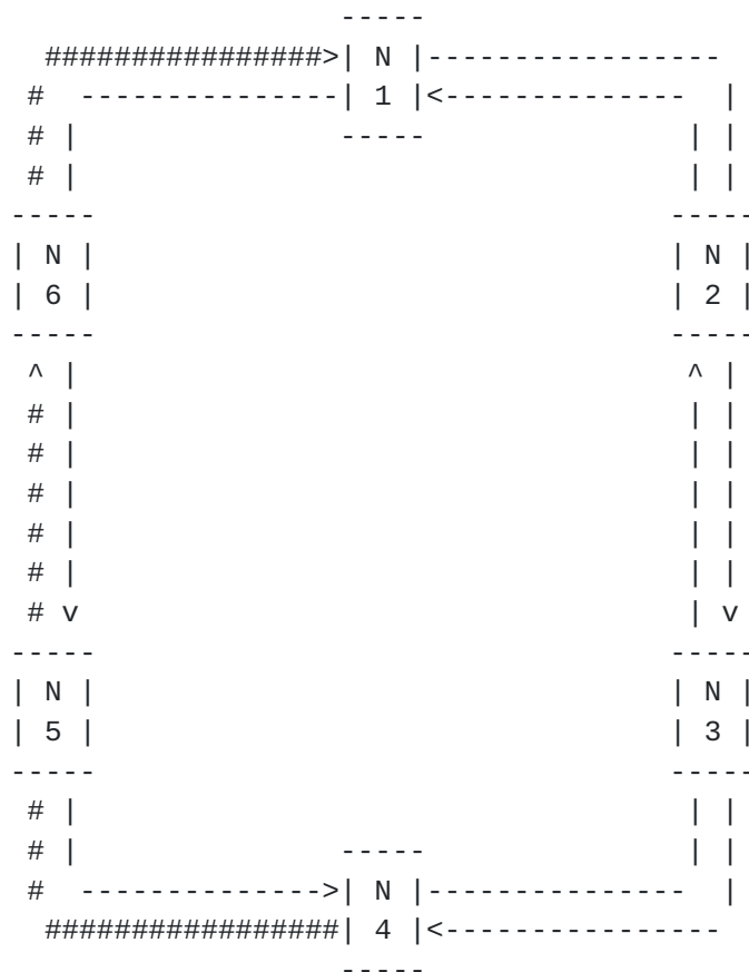
FIGURE 4. Data path before wrap, N4 -> N1
