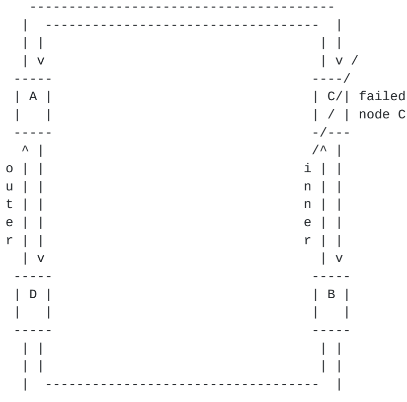
FIGURE 23. An SRP Ring with a failed node
