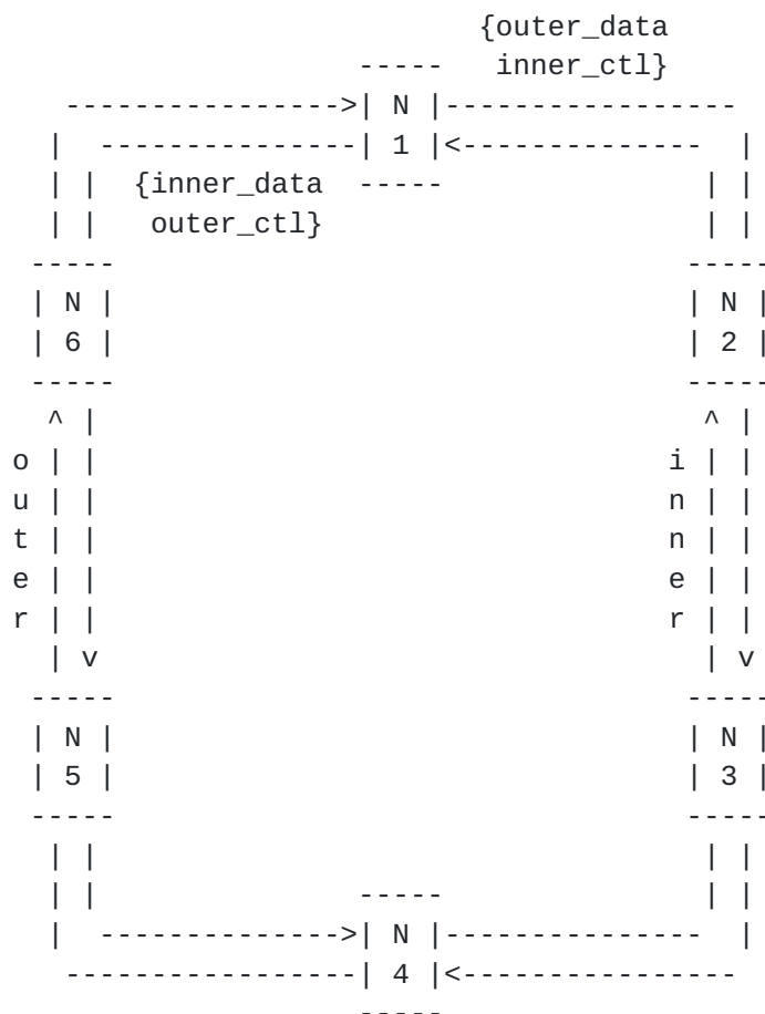
FIGURE 1. Ring Terminology
