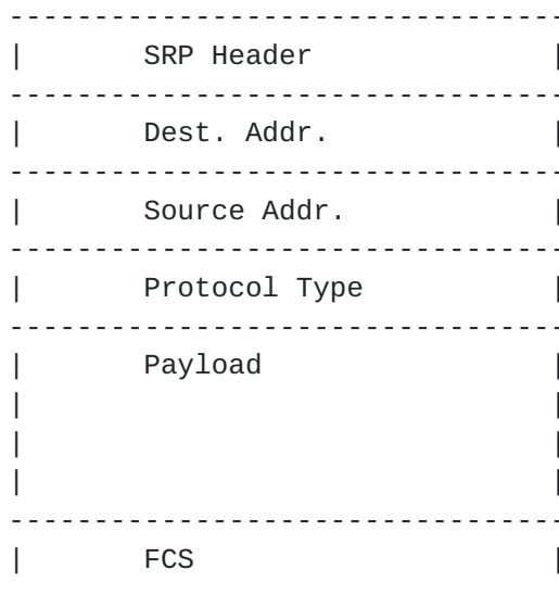
FIGURE 7. Overall Packet Format
