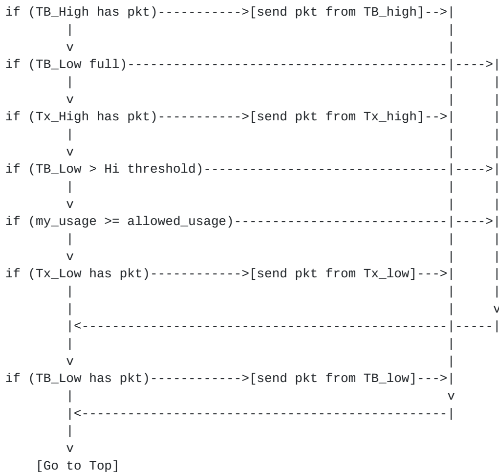
FIGURE 17. SRP transmit flowchart
