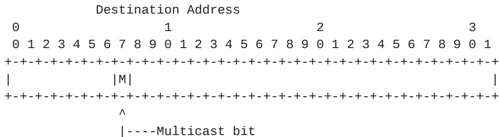
FIGURE 12. Multicast bit position
