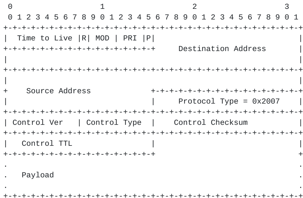
FIGURE 11. Control Packet Format
