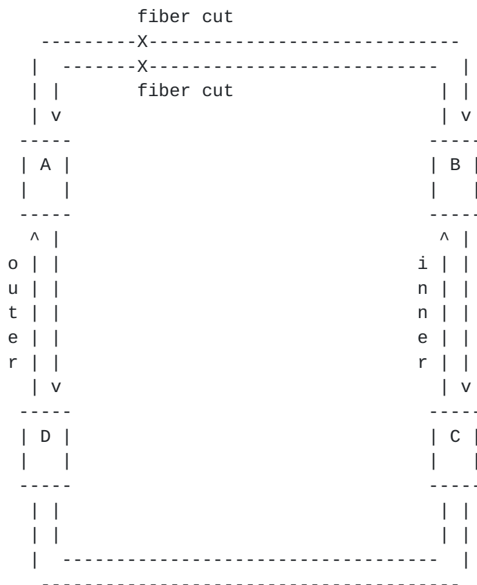
FIGURE 22. An SRP Ring with bidirectional fiber cut
