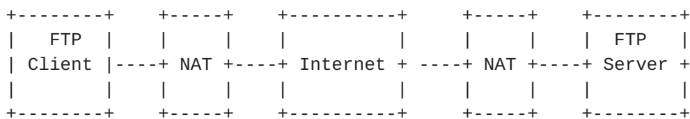
Figure 3: FTP Server and Client Behind NAT
