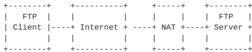
Figure 2: FTP Server Behind NAT
