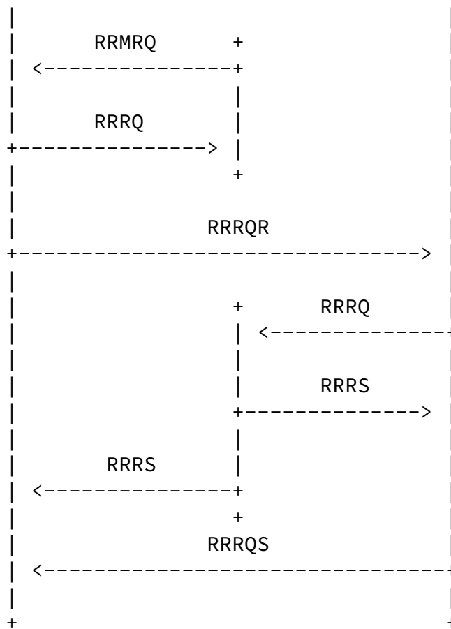
Figure 11: Resource modification sequence (management server trigger)
