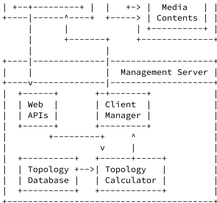
Figure 2: System component
