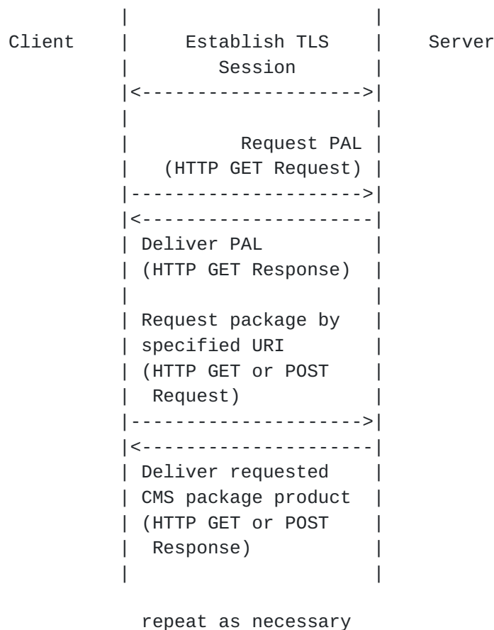
Figure 1 - /pal Message Sequence
