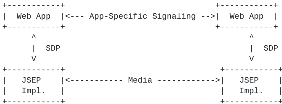
Figure 1: JSEP Signaling Model
