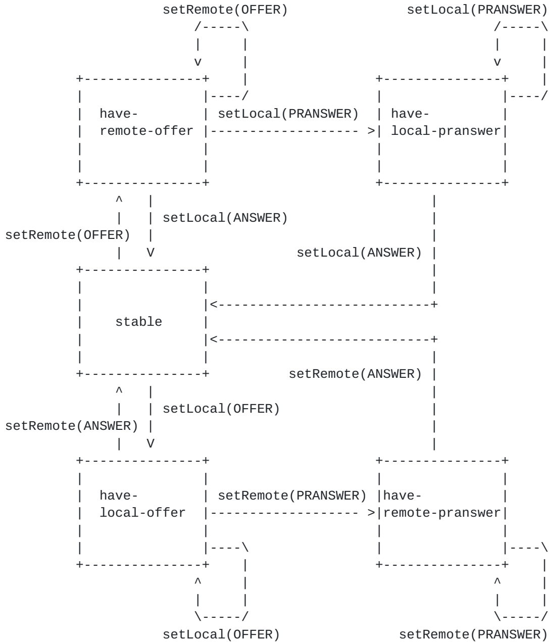
Figure 2: JSEP State Machine
