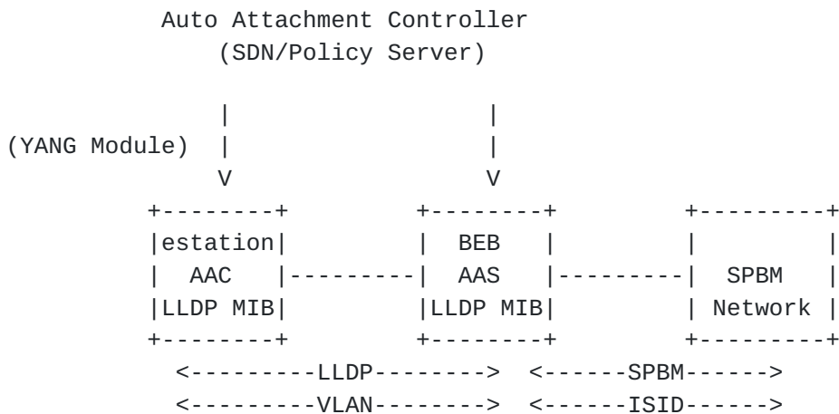
Figure 1: LLDP exchanges trigger IS-IS SPBM announcements
