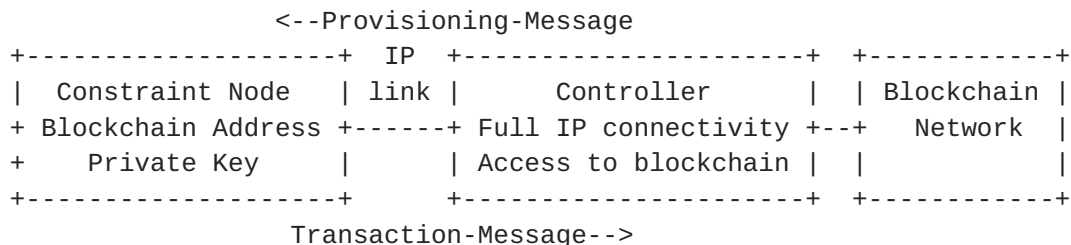
Figure 1. Functional architecture for the Blockchain Transaction Protocol for Constraint Nodes
