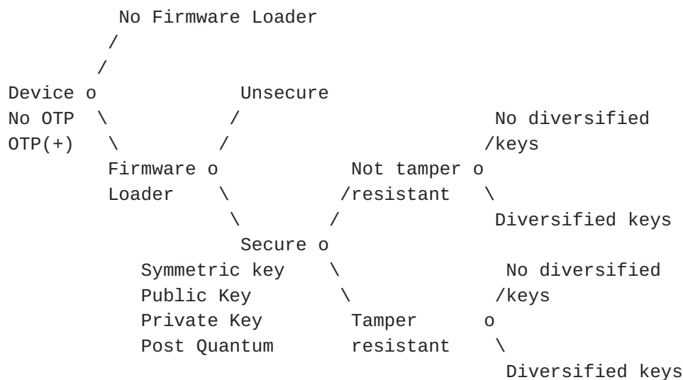
Figure2. Security classes
