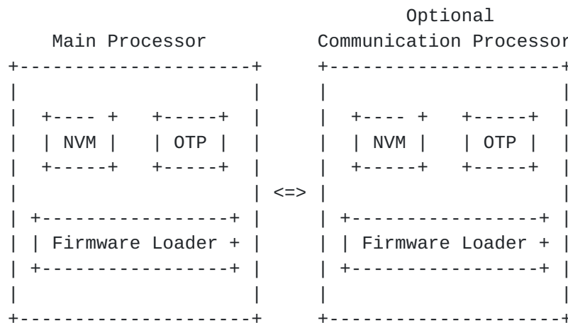
Figure1. Device architecture
