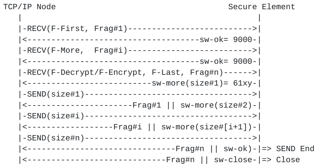
Figure 9. Decryption/Encryption operations.
