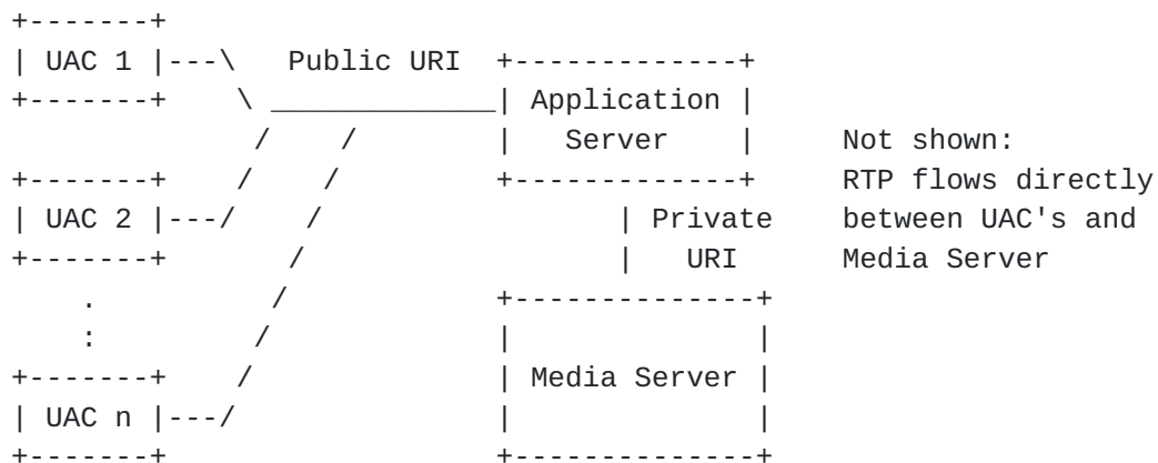
Figure 4: Conference Model
