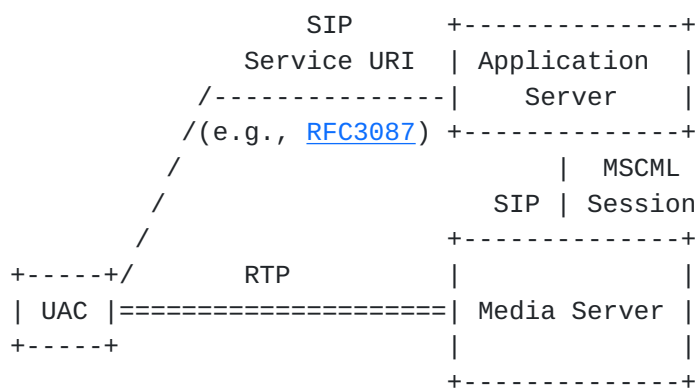
Figure 14: IVR Model
