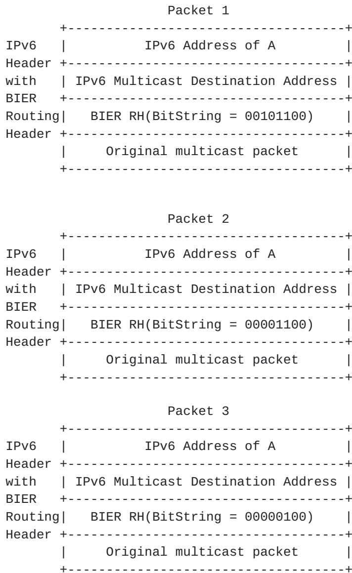
Figure 2: All nodes in BIER domain support BIER Routing Header
