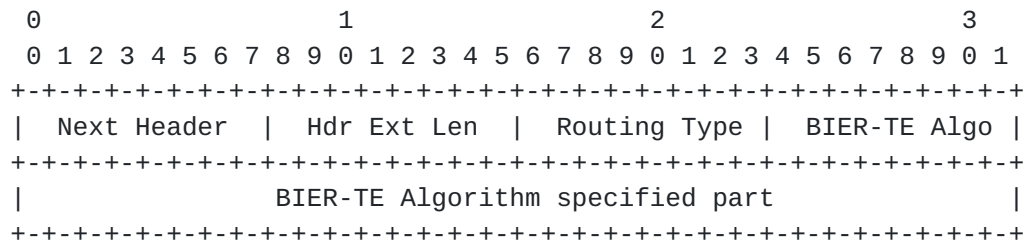
Figure 1: The format of BIER Routing Header
