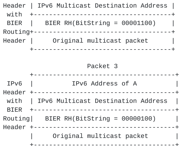
Figure 3: Some nodes in BIER domain do not support BIER Routing Header
