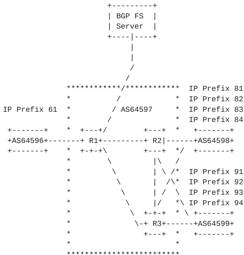
Figure 1: Redirect the traffic using Flowspec
