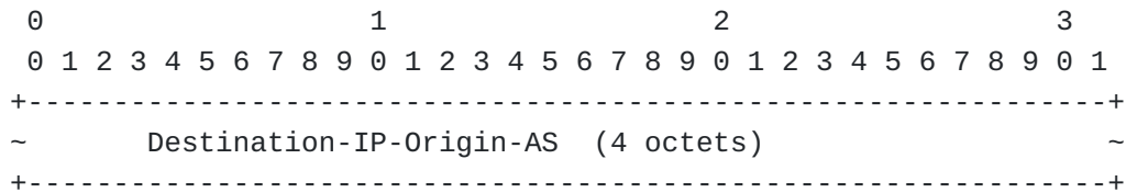
Figure 2: Destination-IP-Origin-AS
