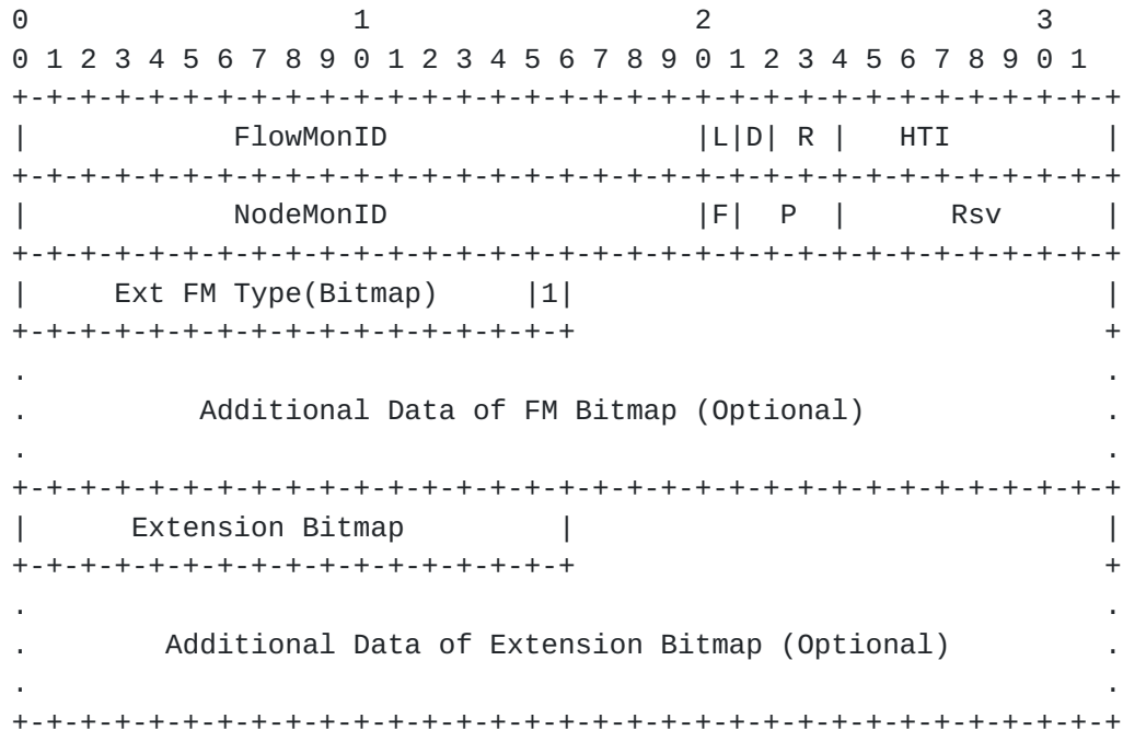
Figure 3: Extension Bitmap Format
