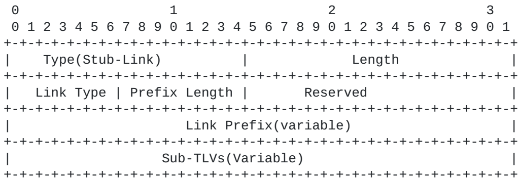
Figure 2: ISIS Stub-Link Sub-TLV
