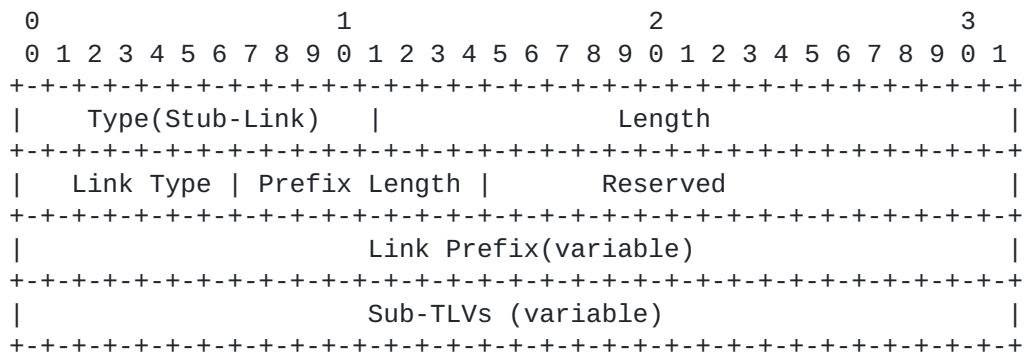
Figure 1: OSPF Stub-Link TLV
