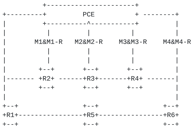
Figure 4: VLAN-Based crossing info Advertisement Procedures for transit PCC and egress PCC
