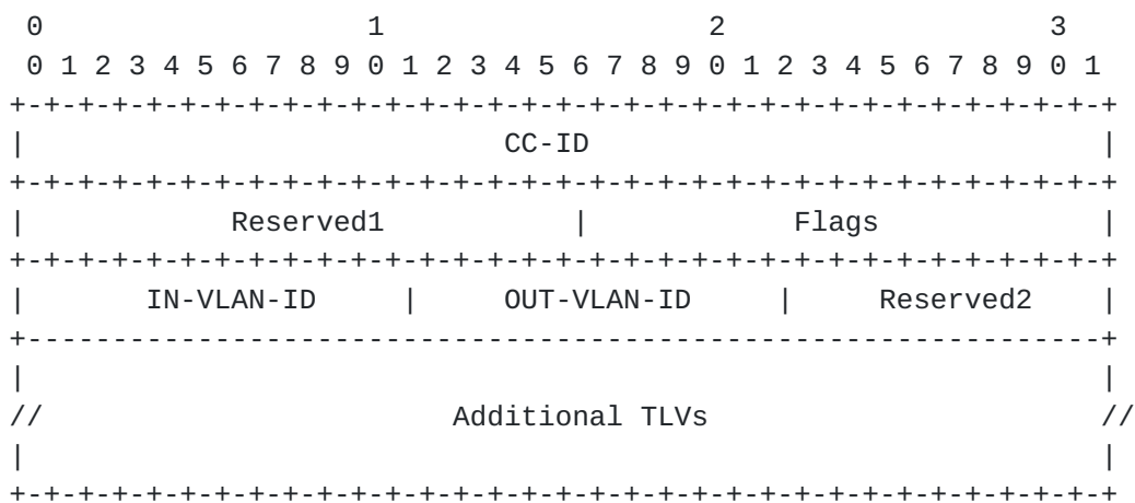
Figure 6: VLAN Crossing CCI Object
