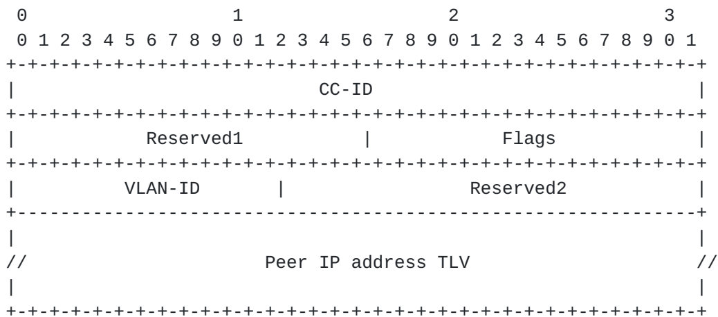
Figure 5: VLAN forwarding CCI Object
