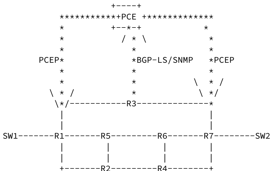
Fig.3 PCE based framework for Multi-BGP deployment
