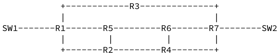
Fig.2 Dual-BGP Framework for large scale network
