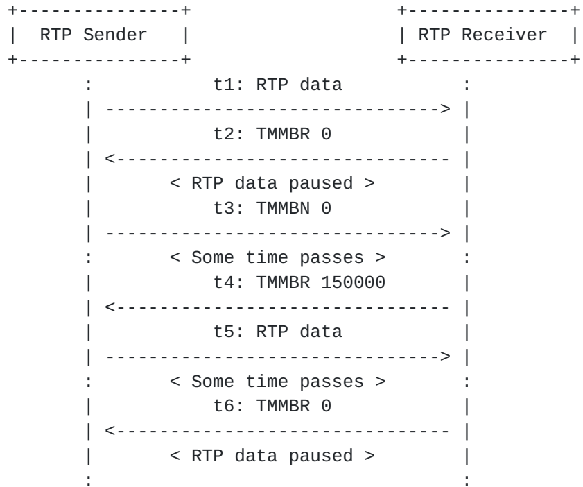
Figure 14: TMMBR Pause and Resume in Point-to-Point
