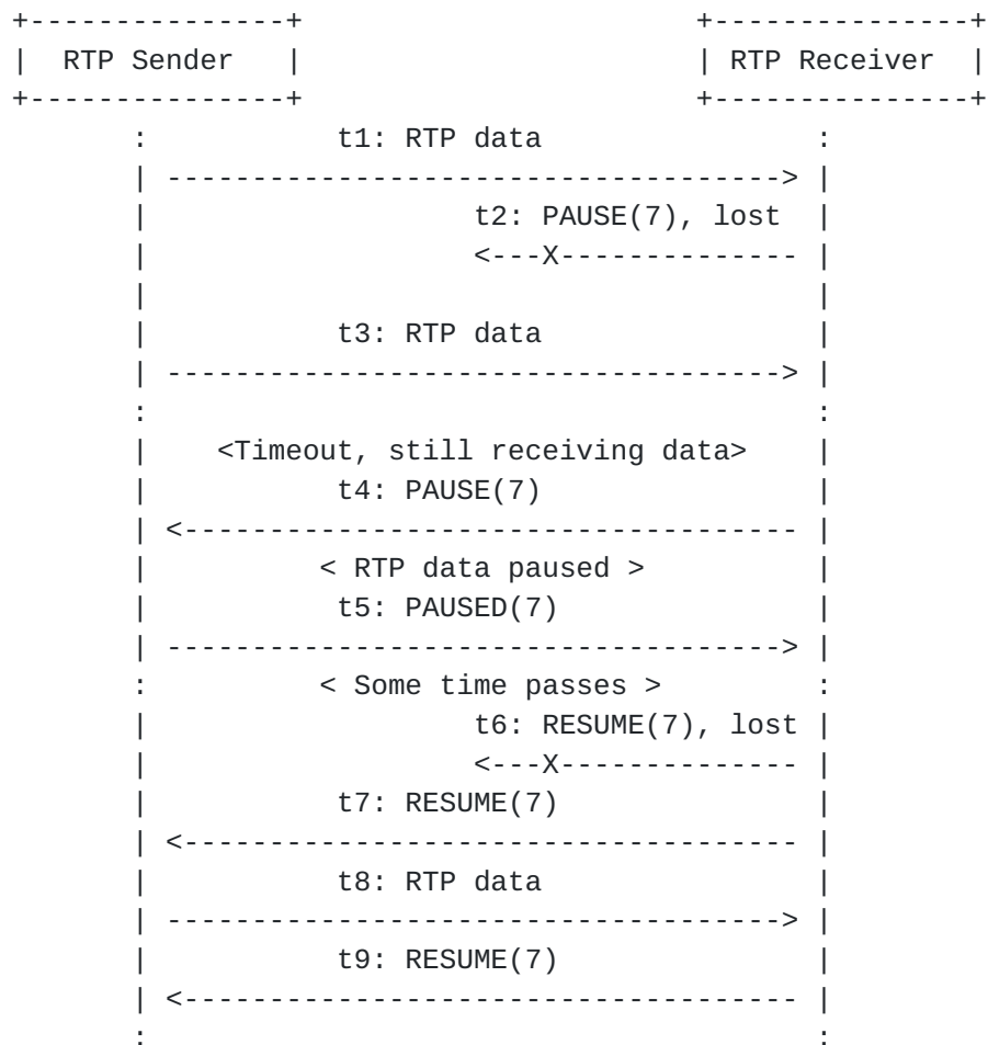
Figure 15: Pause and Resume Operation With Messages Lost
