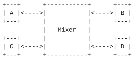
Figure 2: RTP Mixer in Unicast-only
