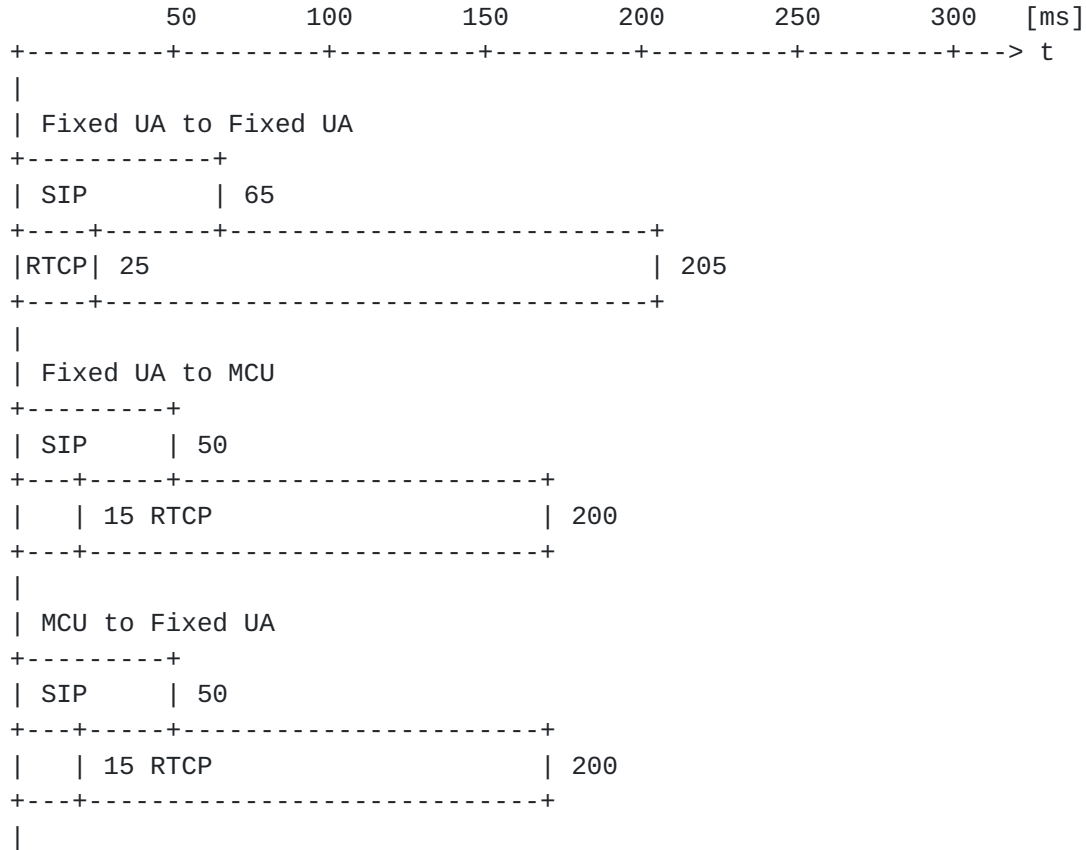
Figure 7: Fixed Access Transmission Delay Comparison
