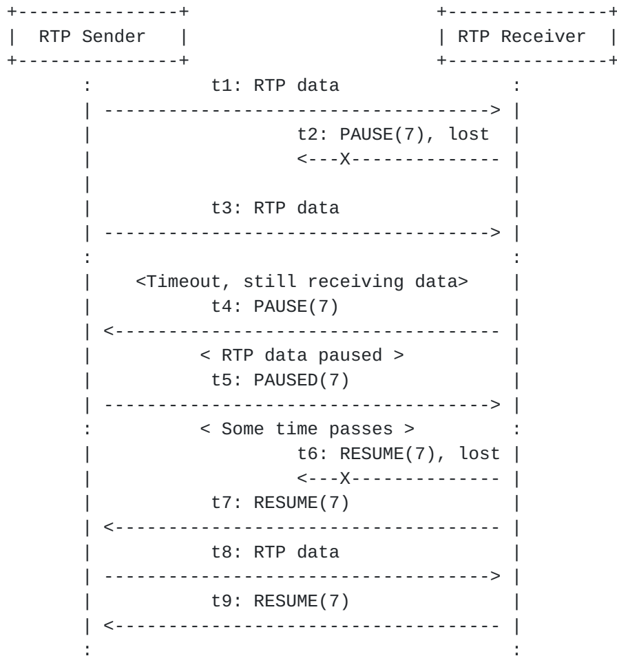
Figure 15: Pause and Resume Operation With Messages Lost
