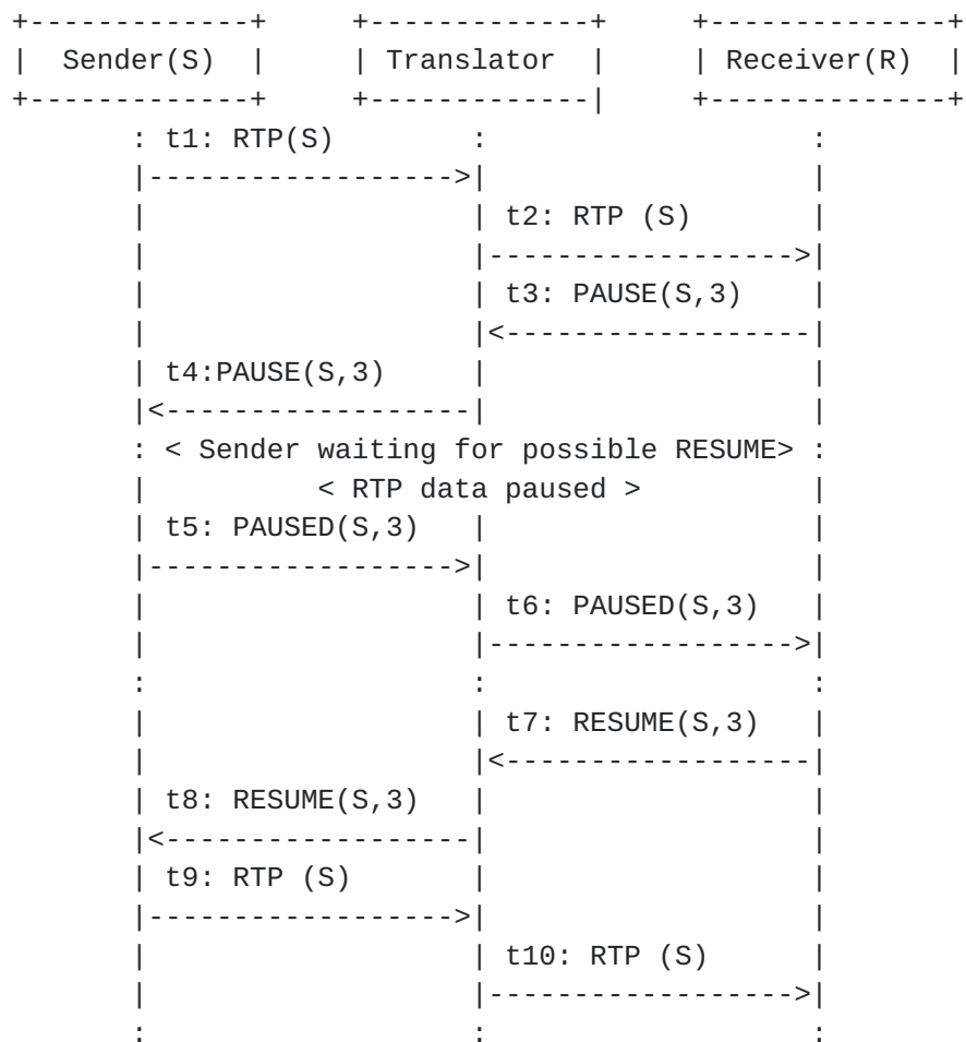
Figure 18: Pause and Resume Operation Between Two Participants Using a Translator
