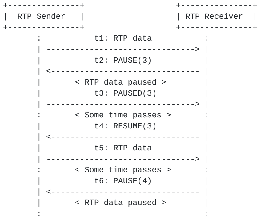
Figure 13: Pause and Resume Operation in Point-to-Point
