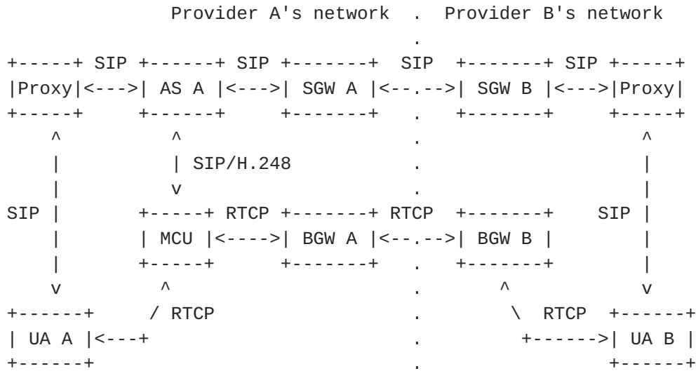
Figure 4: Comparison Signaling Topology
