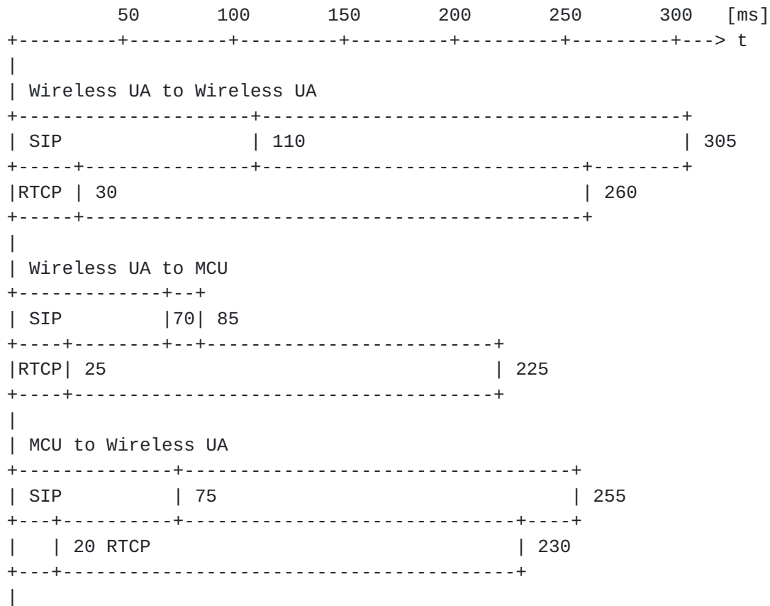
Figure 6: Mobile Access Transmission Delay Comparison
