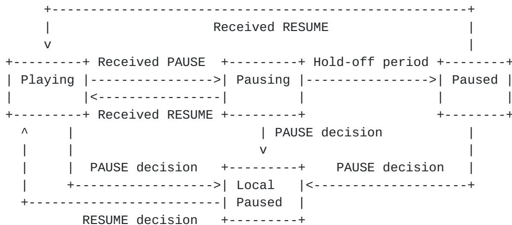
Figure 8: RTP Pause States
