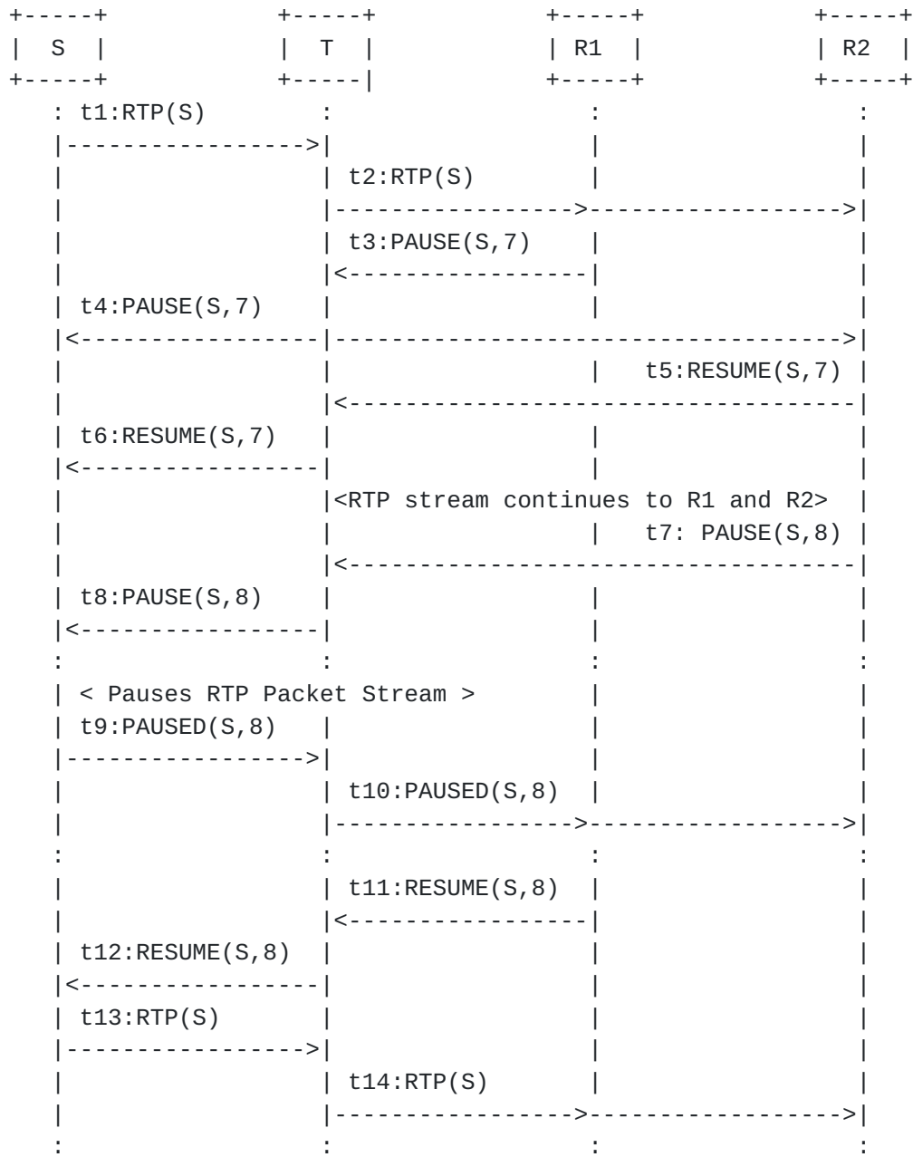
Figure 19: Pause and Resume Operation Between One Sender and Two Receivers Through Translator
