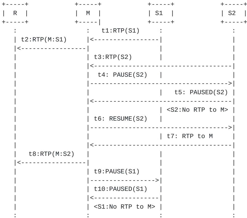
Figure 17: Pause and Resume Operation for a Voice Activated Mixer
