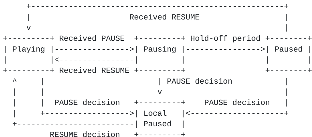
Figure 8: RTP Pause States
