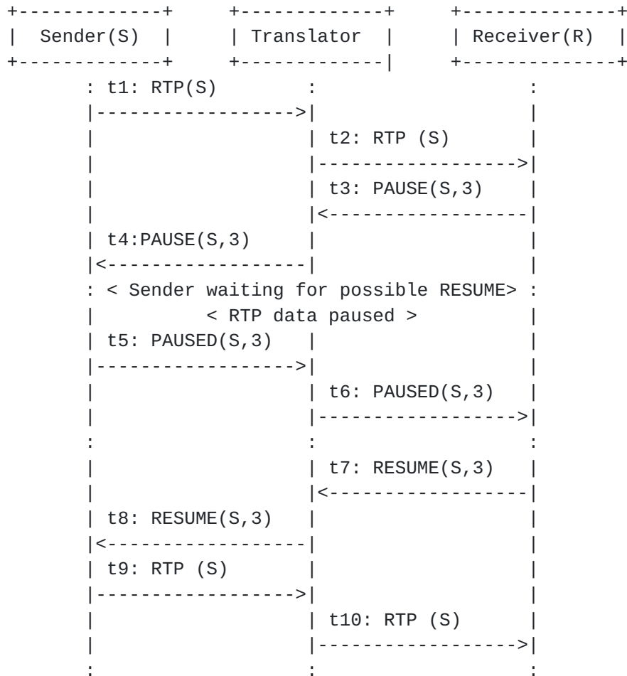
Figure 18: Pause and Resume Operation Between Two Participants Using a Translator
