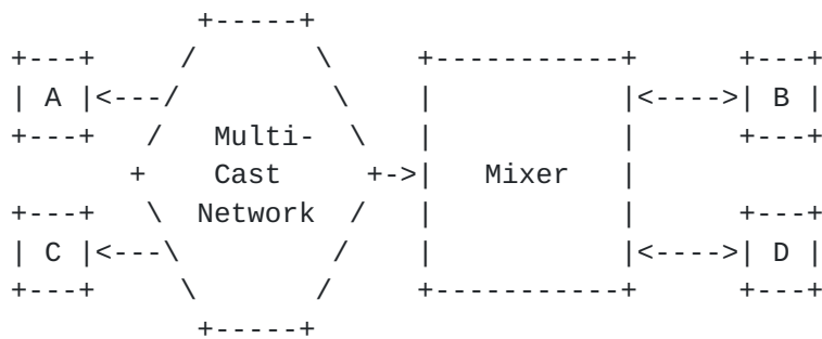
Figure 3: RTP Mixer in Point-to-Multipoint
