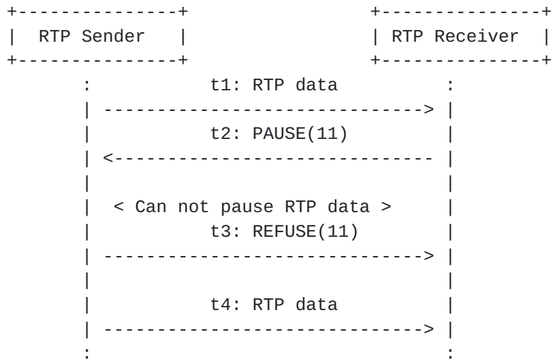
Figure 16: Pause Request is Refused in Point-to-Point
