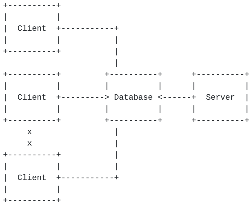
Figure 4: Database Discovery Example
