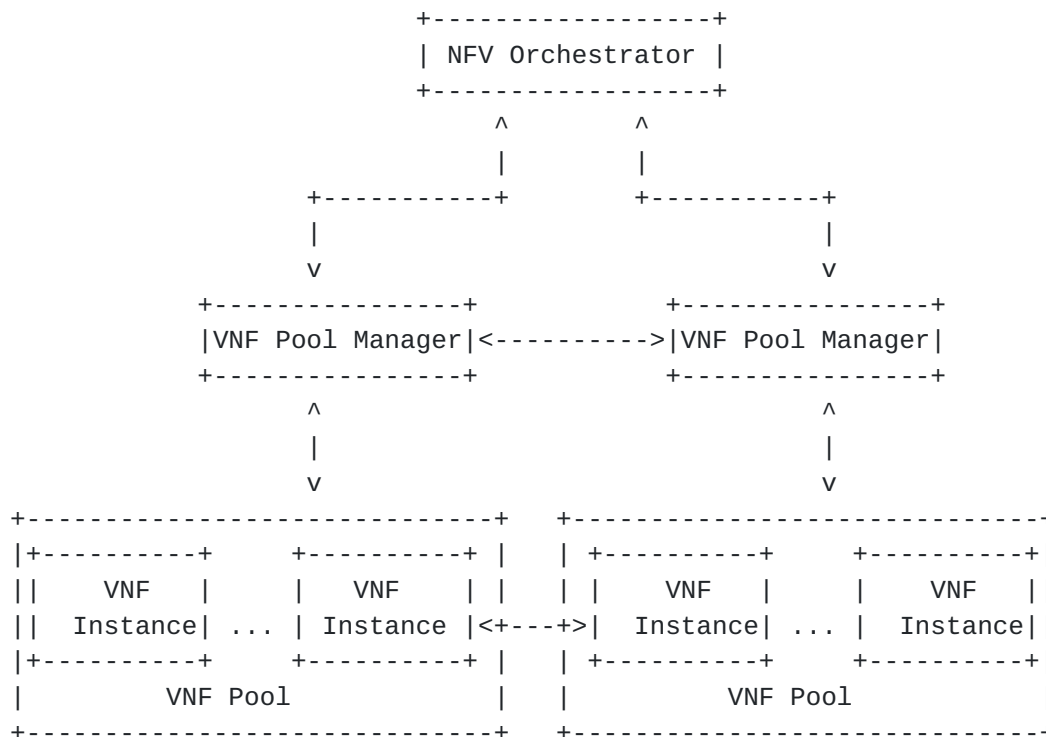
Figure 1: Typical VNF Pool Network Architecture
