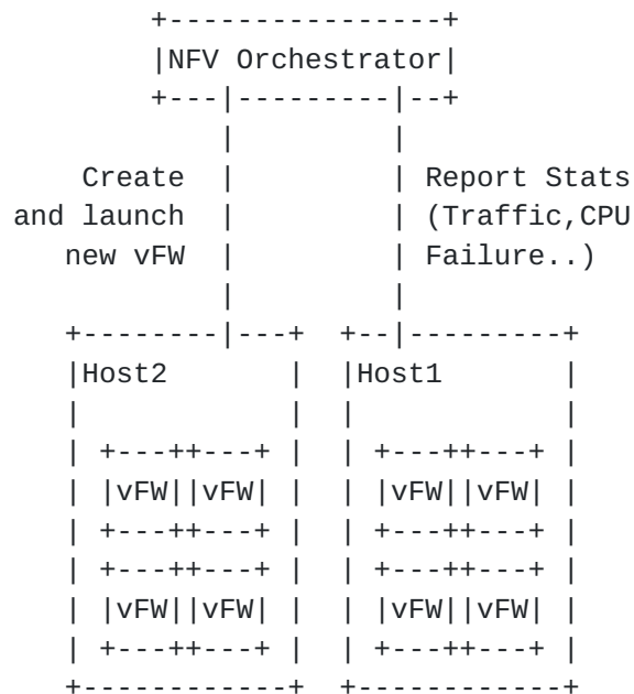
Figure 5: Existing vFW replacement
