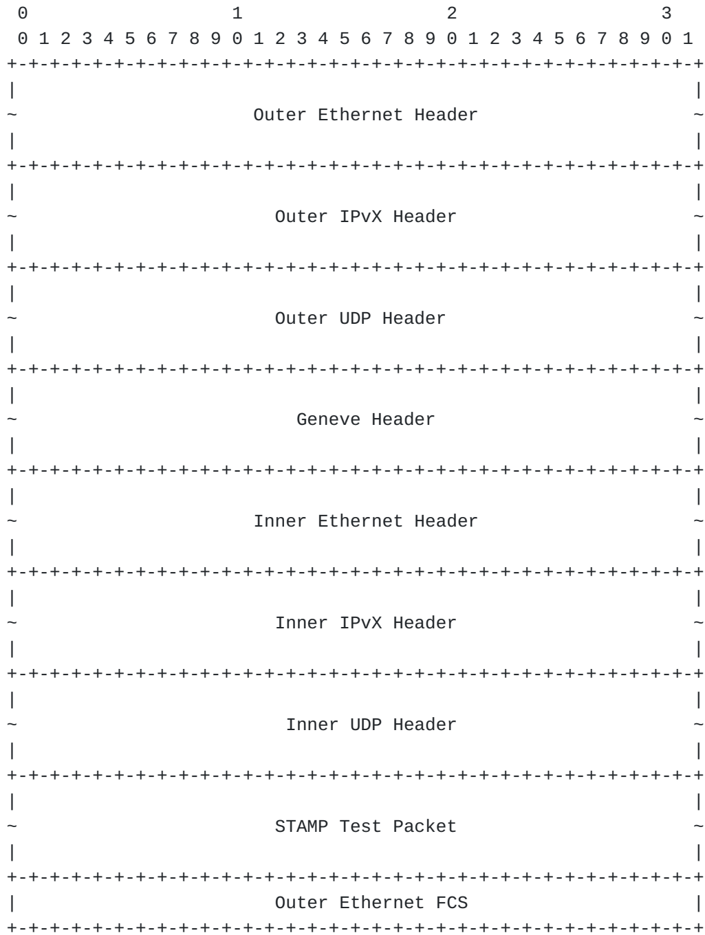
Figure 1: Geneve Encapsulation of PM Packet With the Inner Ethernet/IP/UDP Header
