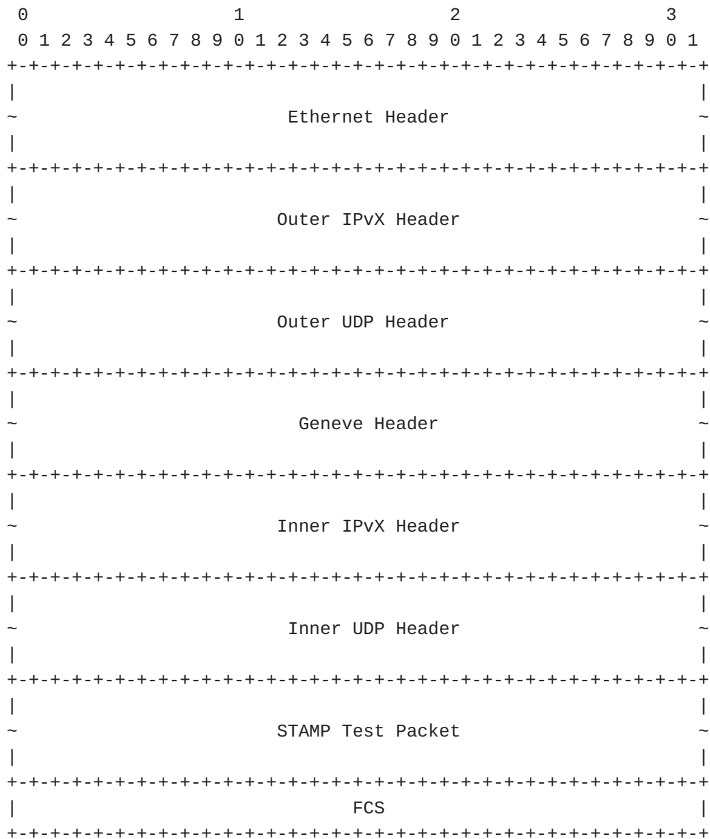
Figure 2: Geneve Encapsulation of PM Packet With the Inner IP/UDP Header
