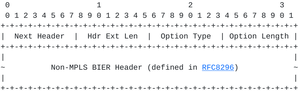
Figure 1: IPv6 BIER Destination Option
