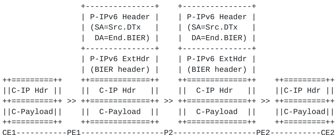
Figure 1: BIERv6 MVPN/GTM Intra-AS
