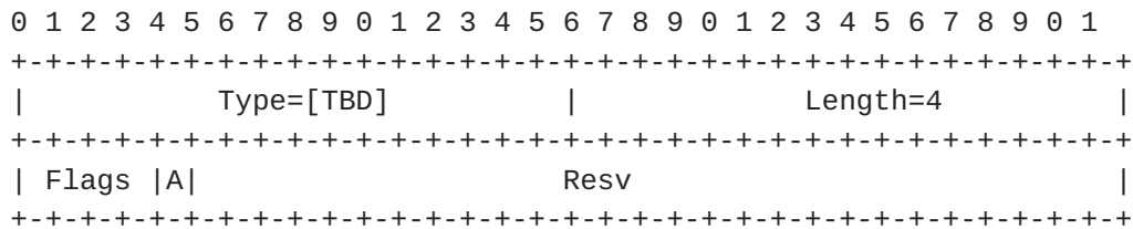
Figure 1 SCHED-BW-ADJUST-CAPABILITY Flags format
