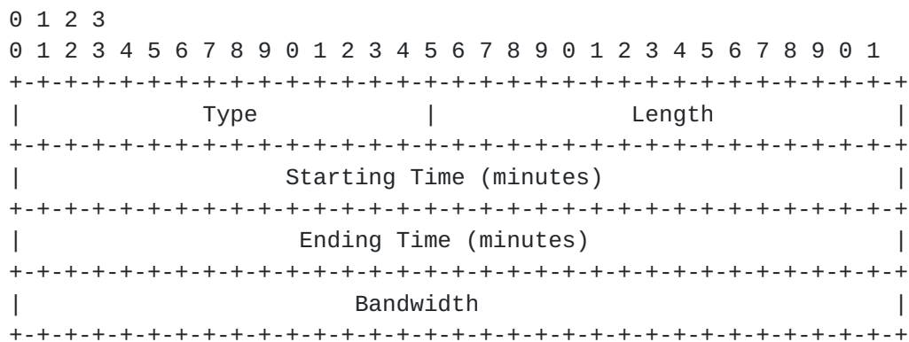
Figure 2 SCHED-BW-ADJUST-ATTRIBUTE TLV format
