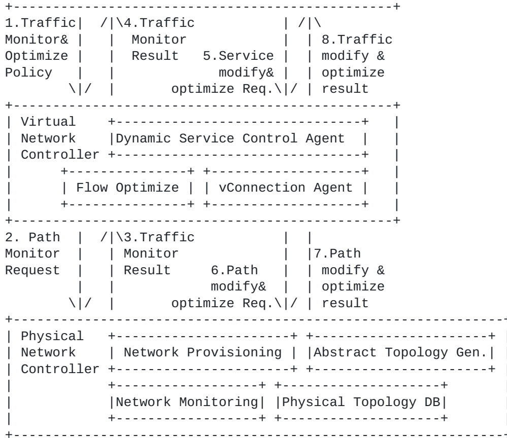
Figure 1 Workflows for dynamic service control based on traffic monitoring
