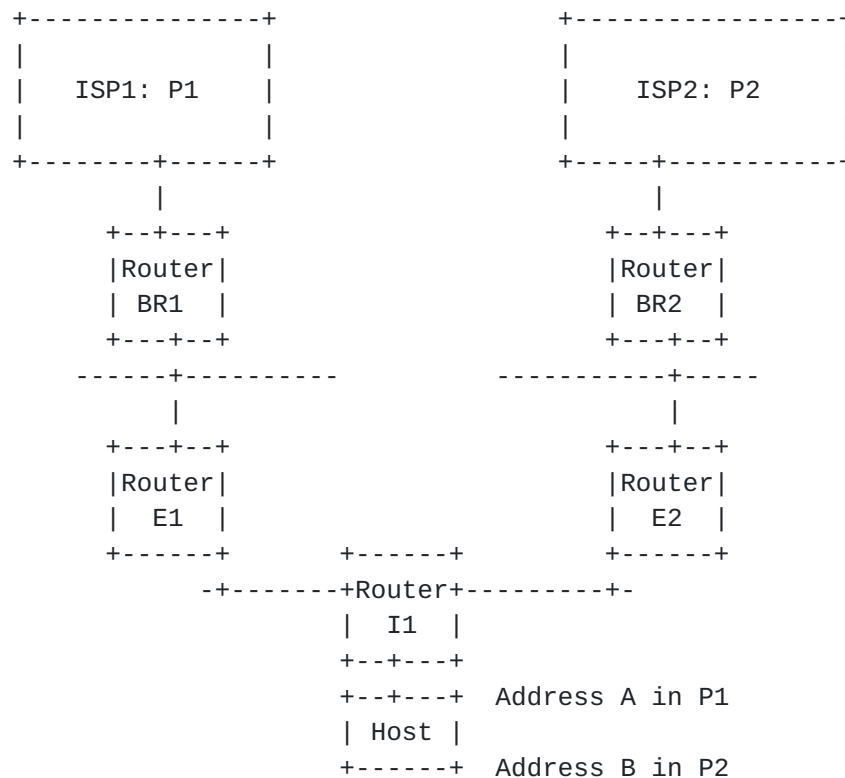
Figure 1: Multi-homing Scenario in Home Networks
