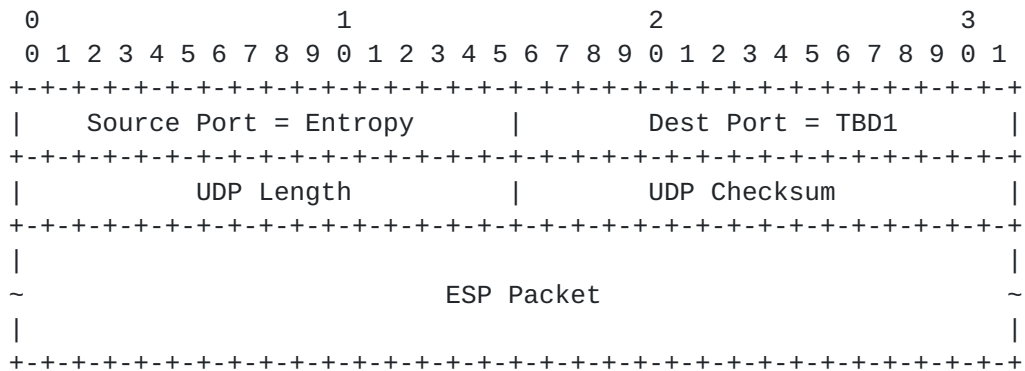
Figure 1: ESP-in-UDP Encapsulation Format
