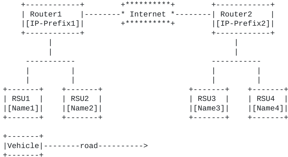
Figure 1: Name and address management architecture
