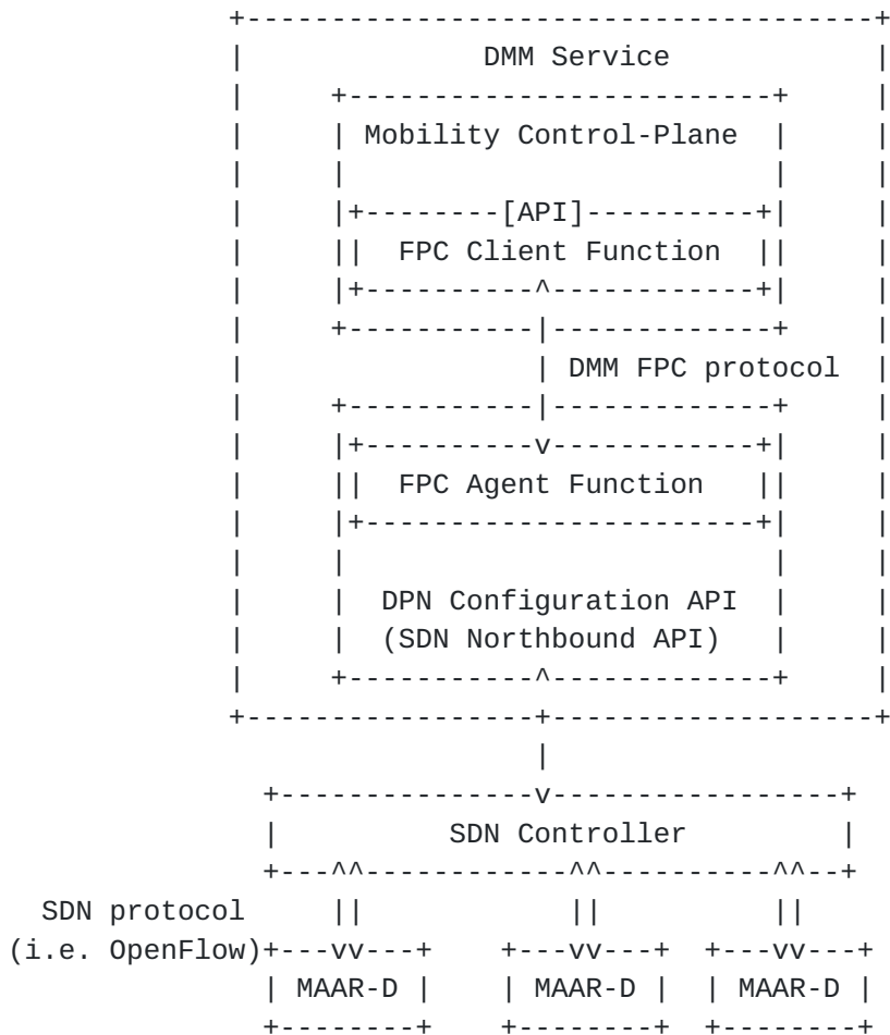
Figure 4. Functional Architecture for Supporting FPC Protocol in SDN-based DMM
