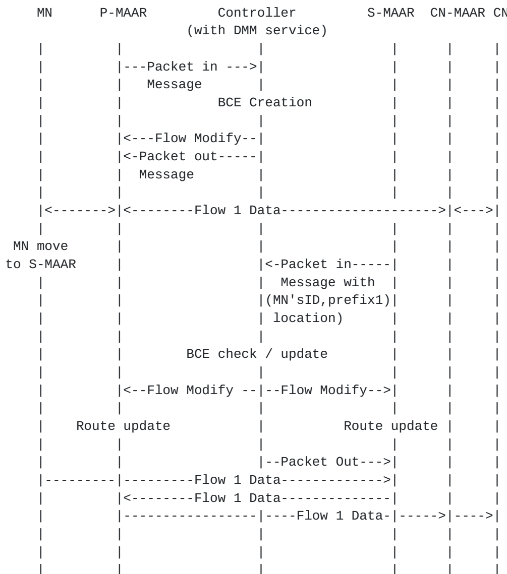
Figure 2. Procedure of DMM with SDN
