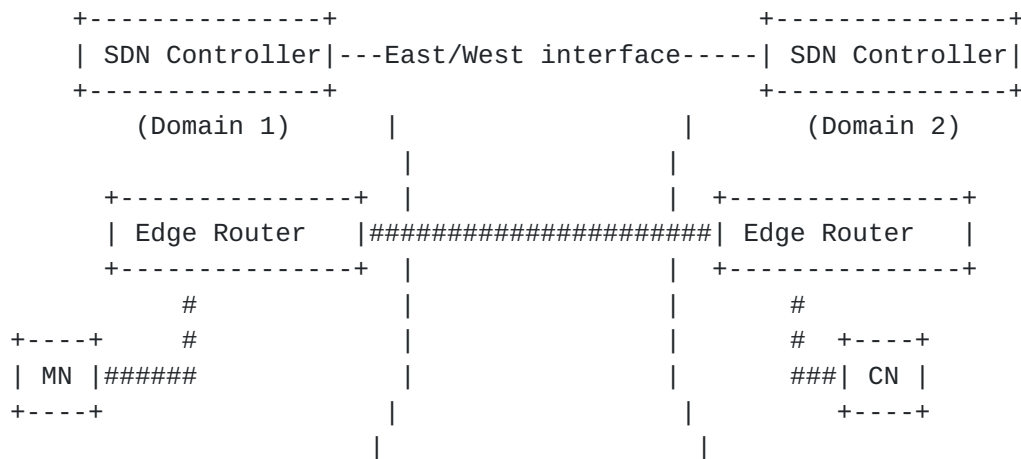
Figure 5. Data flow in Different Domains
