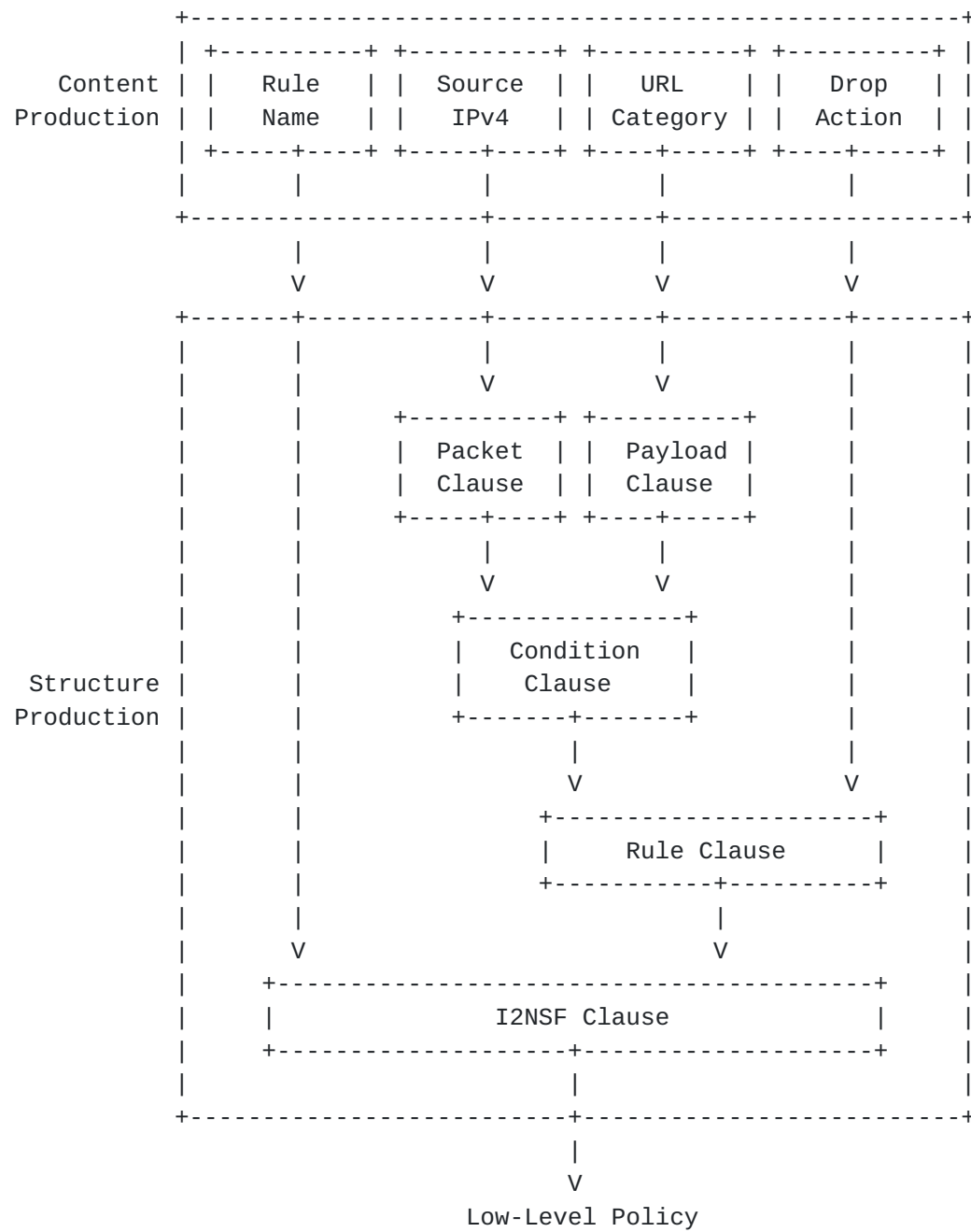
Figure 7: Generator Construction for Web-Filter NSF
