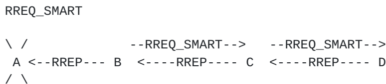
Figure 3: LOADng route discovery from Router A to Router D with Smart Route Request. Router B and Router C have already availalbe routes to Router D
