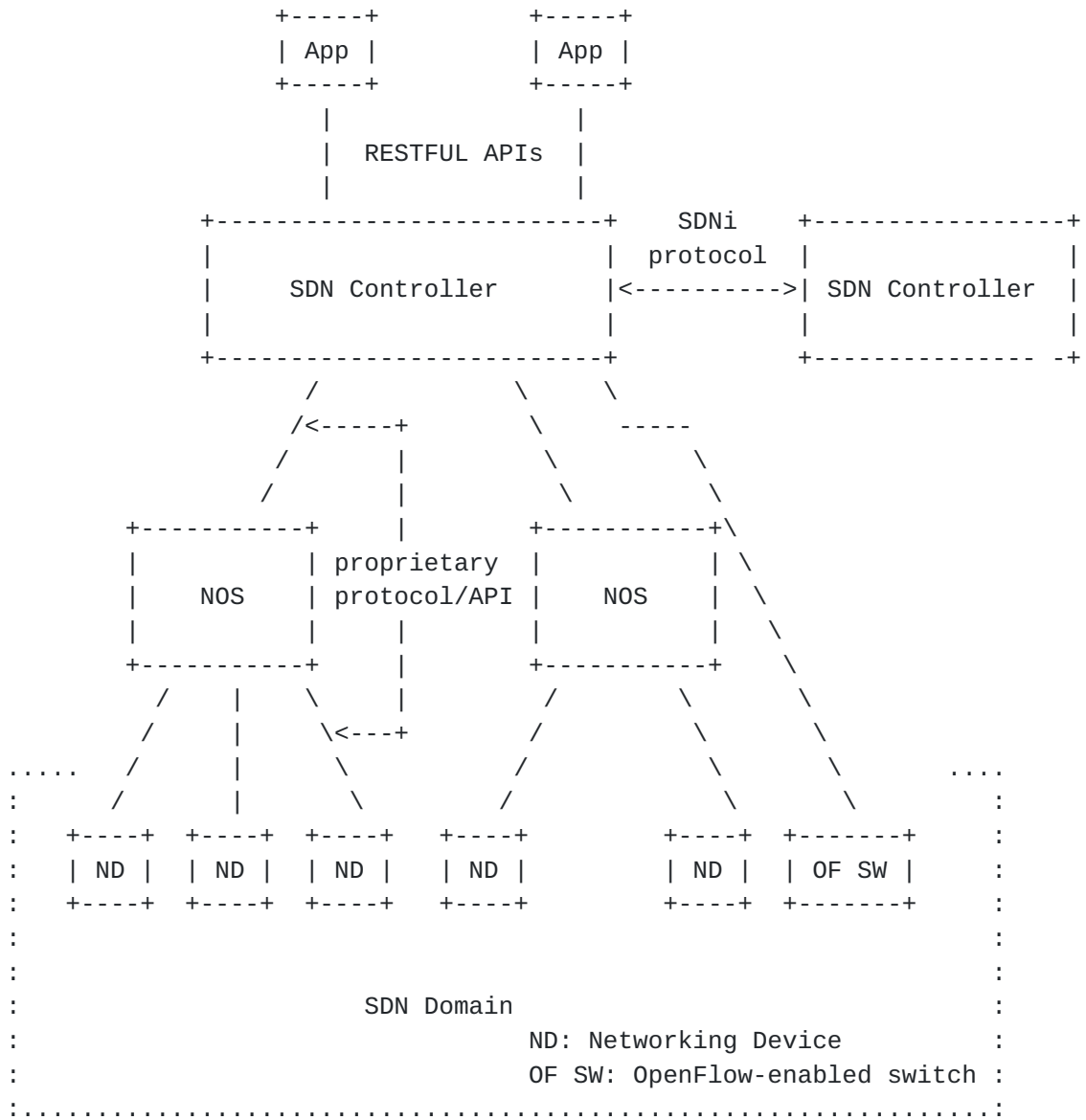
Figure 1: An Architecture For SDN
