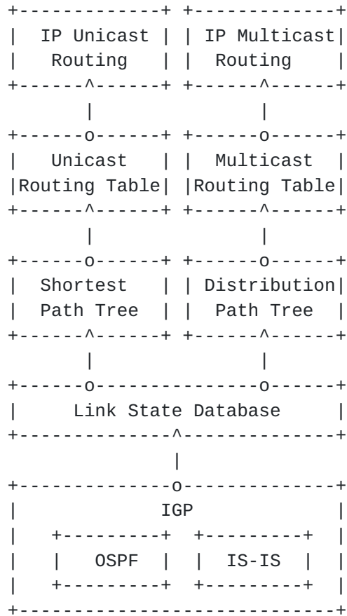
Figure 1: Using an IGP to Route both IP Unicast and Multicast Packets
