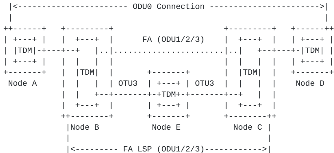
Figure 3b - TDM nested LSP provisioning
