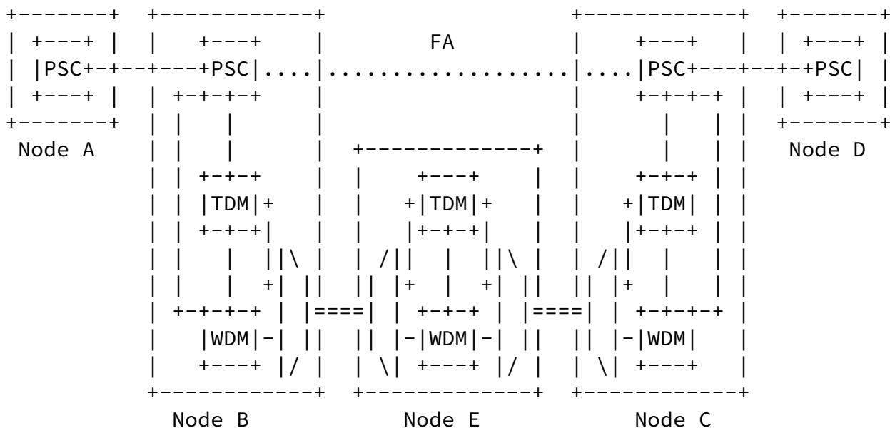
Figure 2 - MLN with multiple ISCs at edge node
