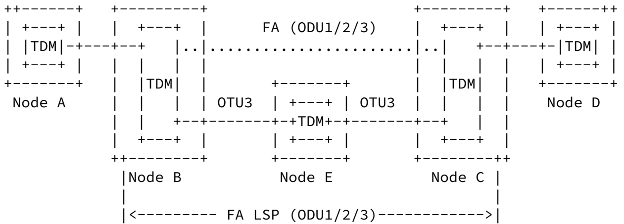
Figure 3b - TDM nested LSP provisioning
