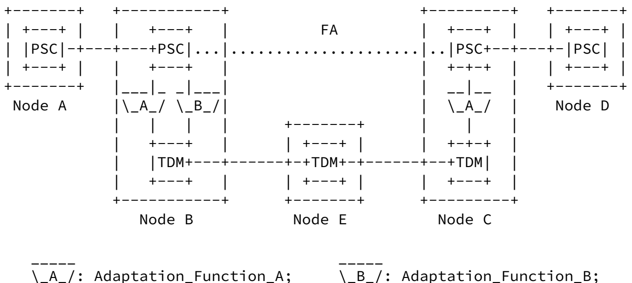
Figure 4 - Selection of adaptation function
