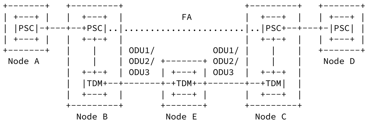
Figure 3a - Multiple switching granularities in server layer
