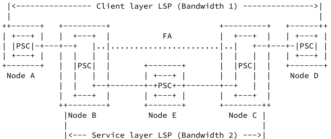
Figure 3c - PSC nested LSP provisioning
