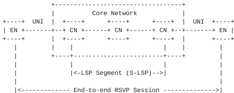
Figure 4 - The Stitching Model
