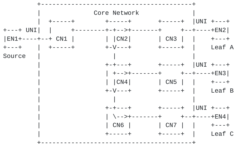
Figure 9 - All CNs support multicast
