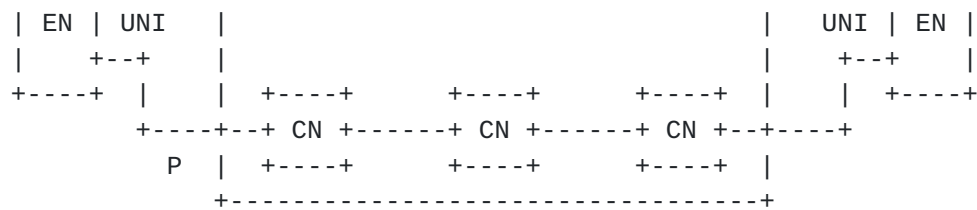
Figure 6 - UNI End-to-End Recovery
