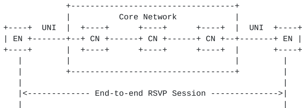
Figure 3 - The Flat Model
