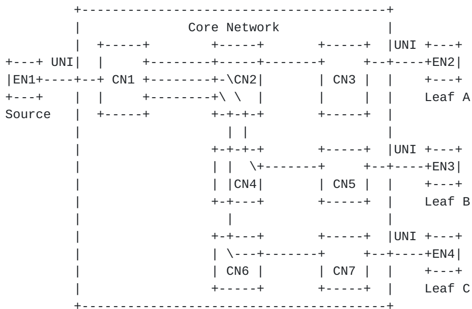
Figure 8 - Only ingress/egress CNs support multicast
