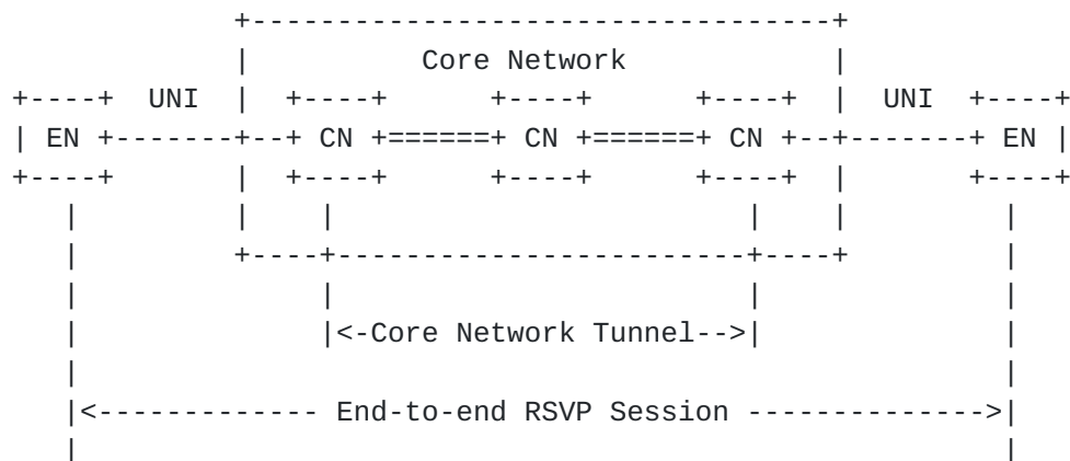
Figure 5 - The Hierarchal Model
