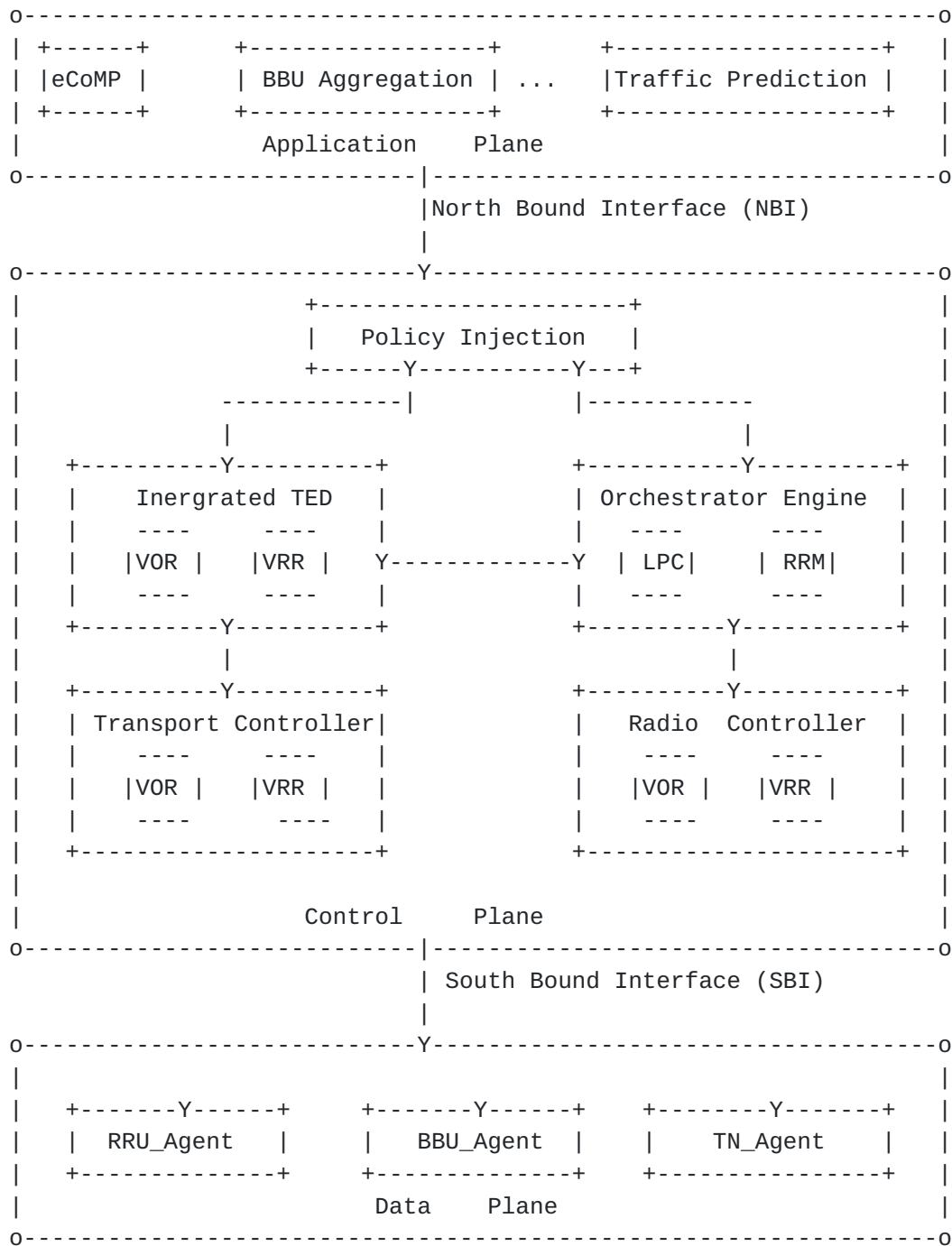
Figure 1: Unified Radio and Optical Control Architecture based on SDN
