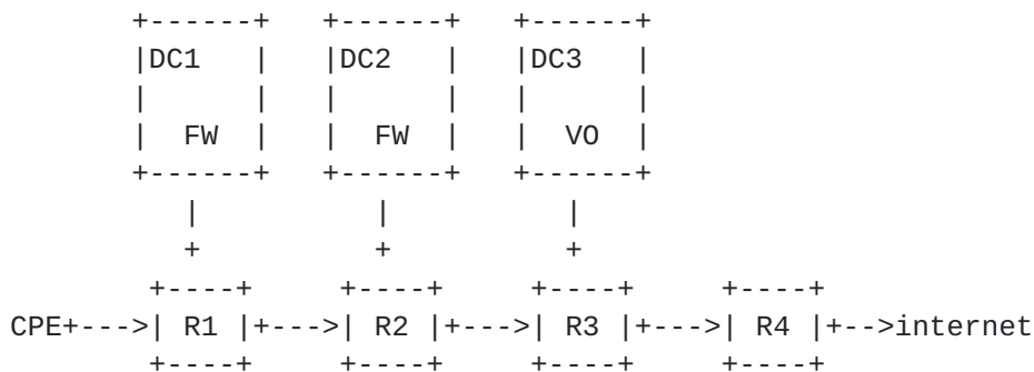
Figure 1: Illustration of Computing-aware SFC
