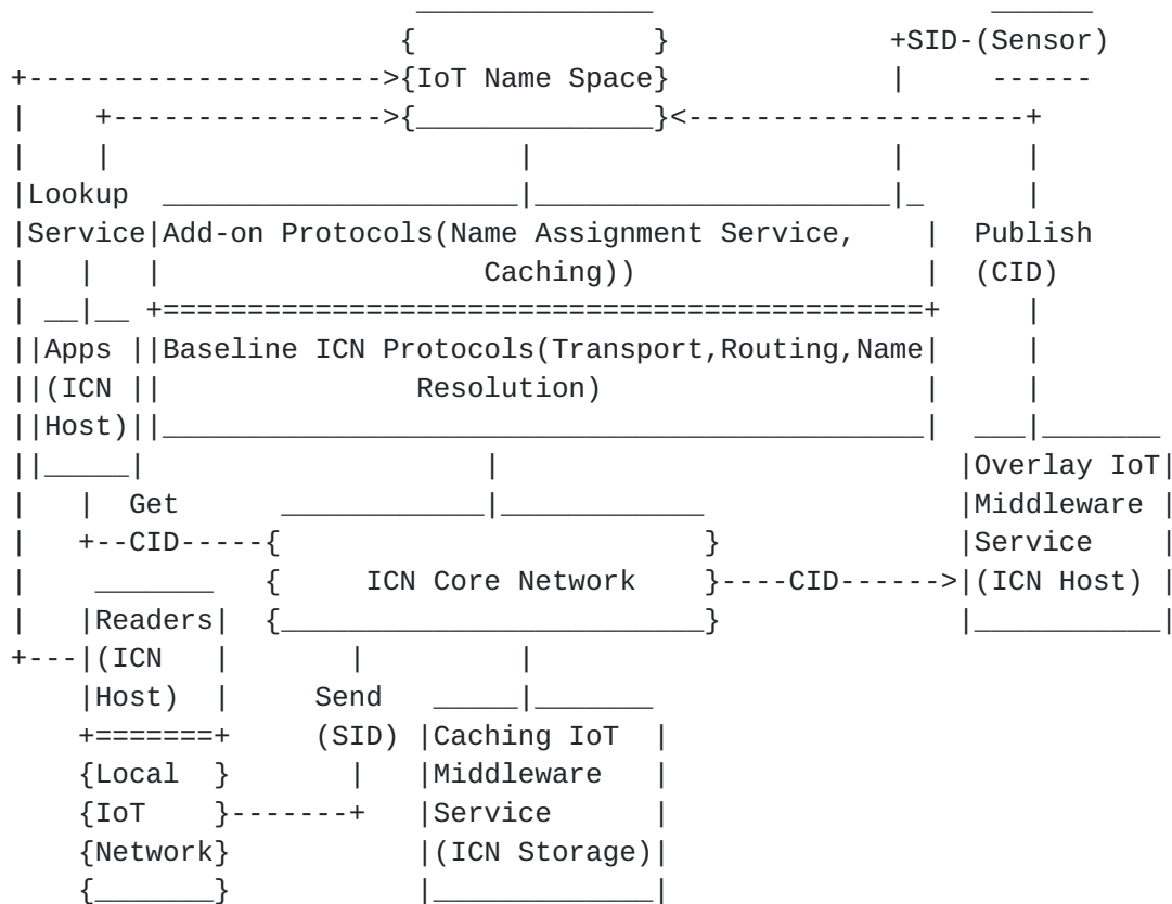
Figure 6: ICN-IoT Data and Services
