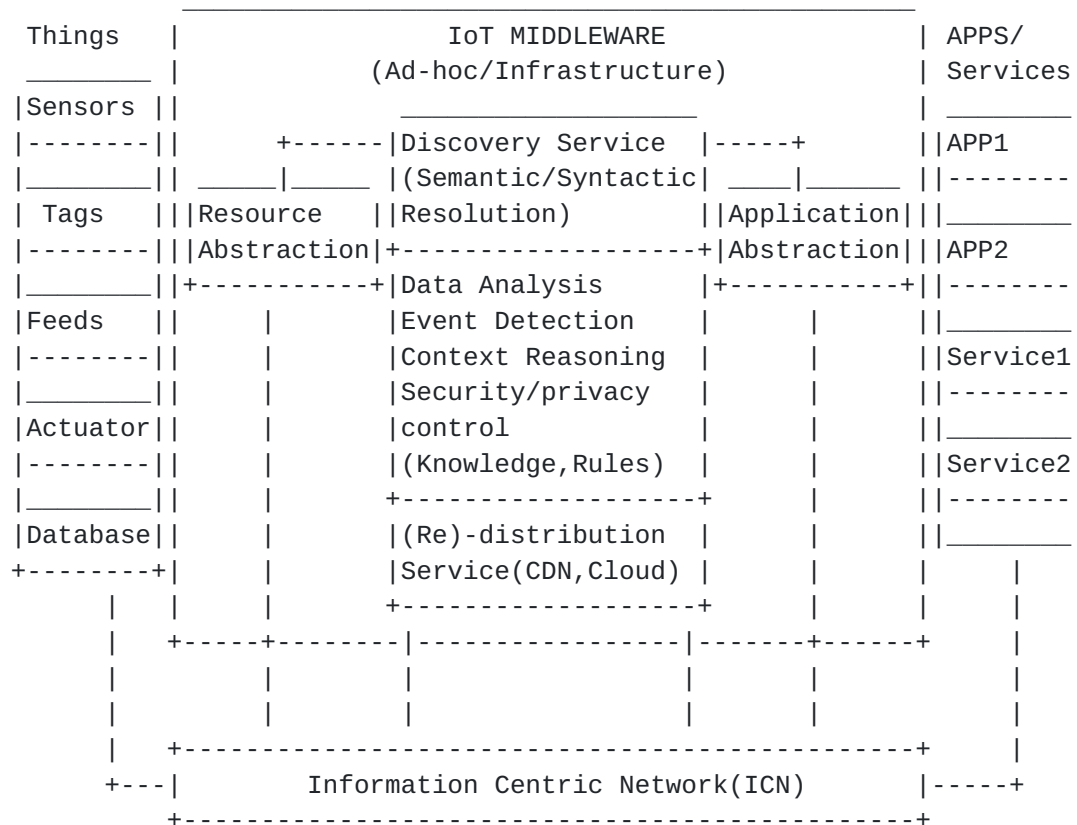
Figure 5: The ICN-IoT Service Middleware
