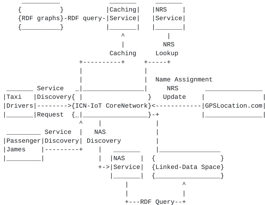
Figure 8: Location context application scenario
