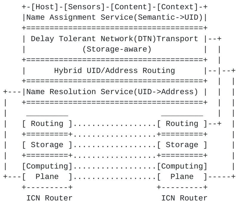
Figure 4: An Example ICN-IoT Architecture
