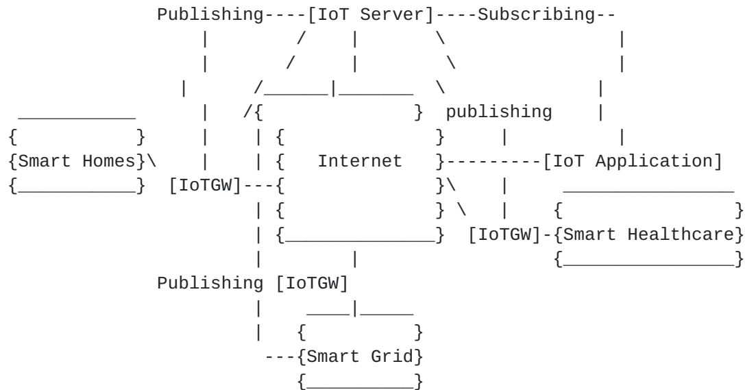
Figure 2: Implementing an open IoT platform through standardized APIs on the IoT gateways and the server
